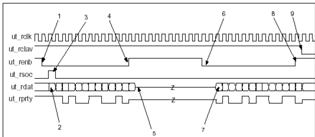
Figure 8: Cell Transfer - Octet Level Transfer
