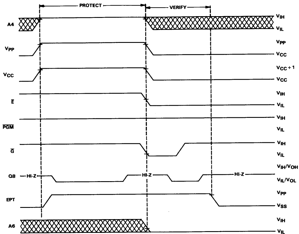
FIGURE 13. EPROM PROTECT TIMING
