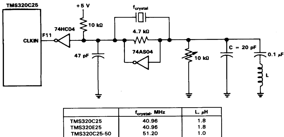
FIGURE 7. EXTERNAL CLOCK OPTION
