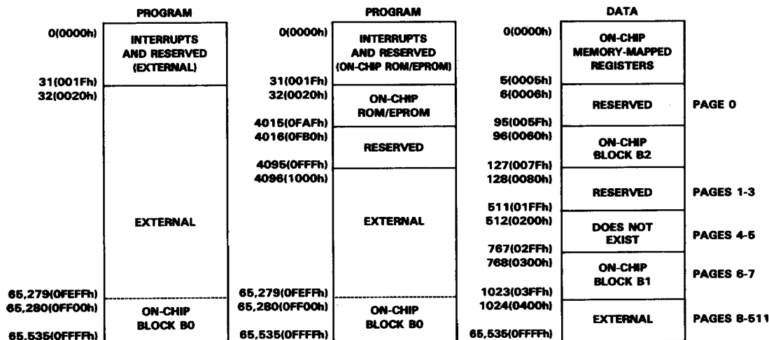
(a) MEMORY MAPS AFTER A CNFD INSTRUCTION
