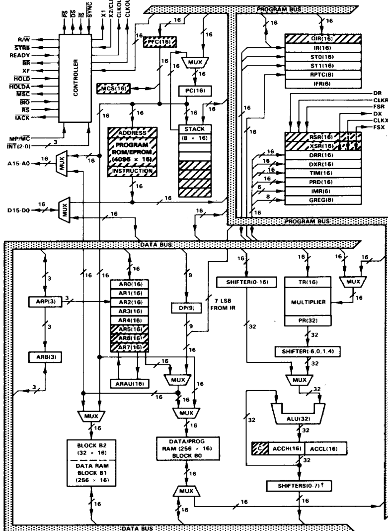
functional block diagram (TMS320C2x)
