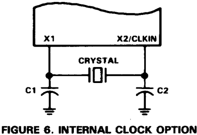
FIGURE 6. INTERNAL CLOCK OPTION
