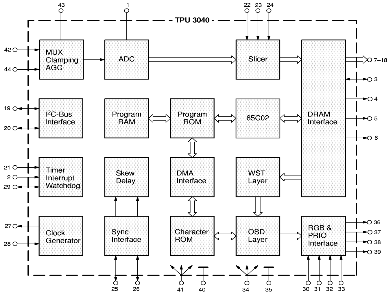
Fig. 2-1: Functional block diagram of the TPU 3040
