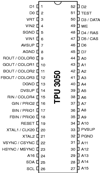
Fig. 3-5: TPU 3050 in 52-pin PSDIP package
