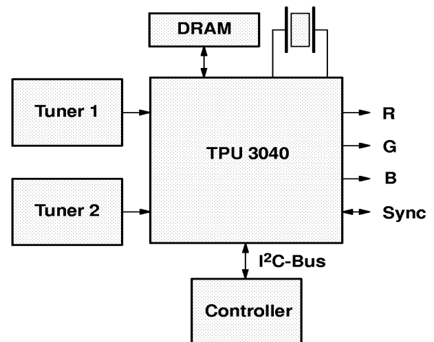
Fig. 2–4: Stand-Alone Application
