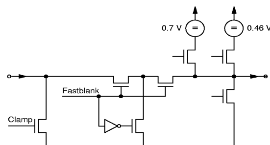
Fig. 3-15: Input/Output Pins 31 to 33 and 37 to 39
