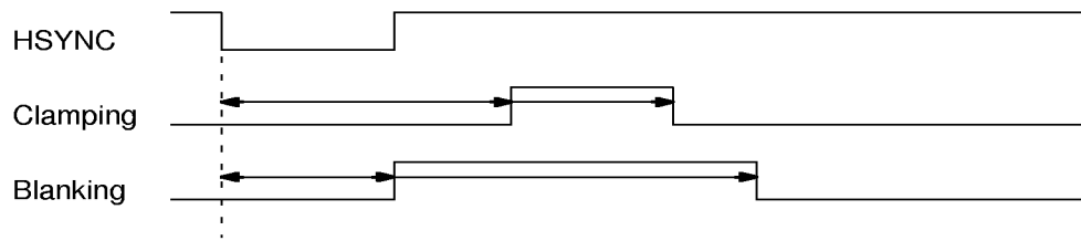
Fig. 2–6: Internal Timing
