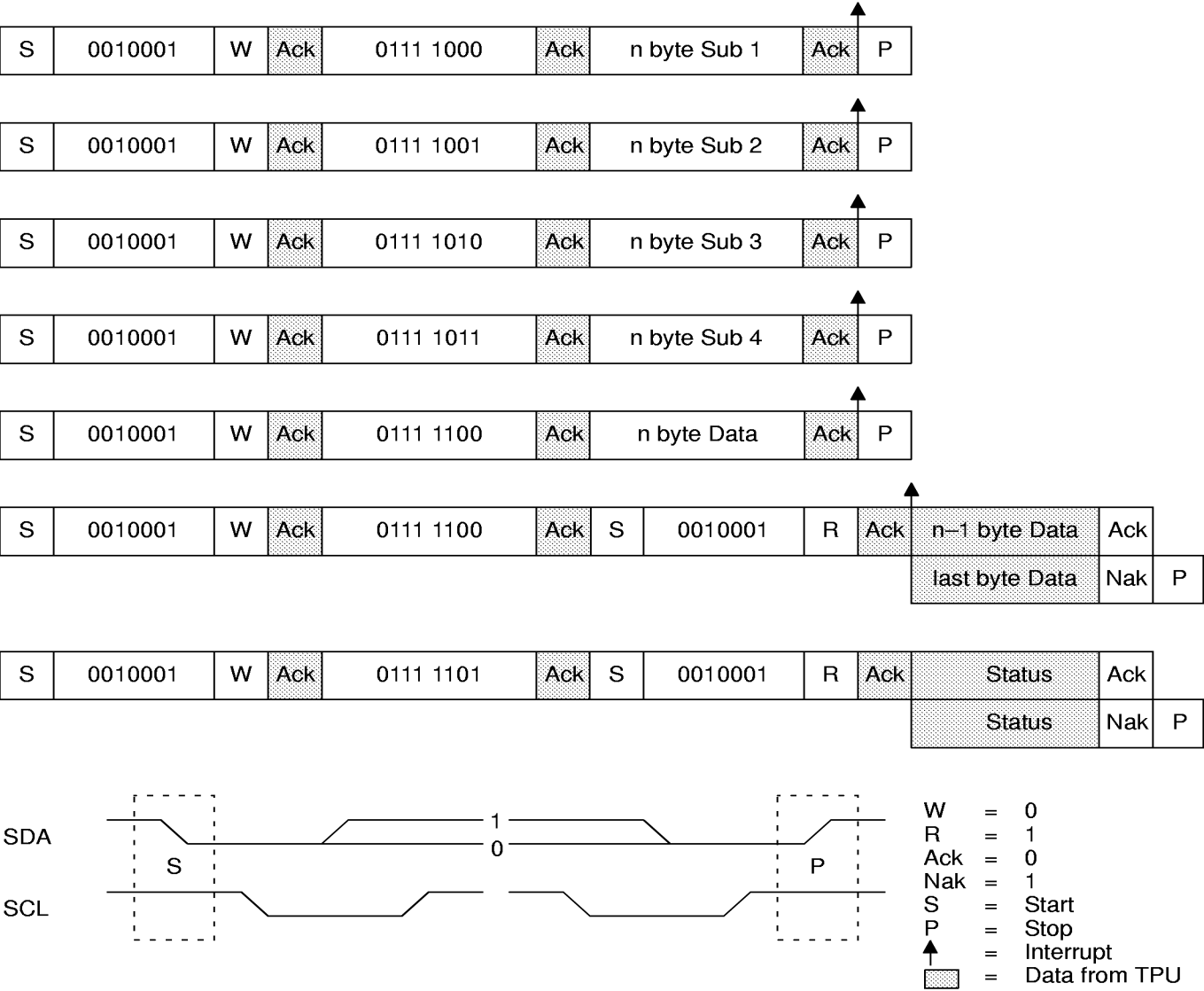
Fig. 4–3: I 2 C-bus Protocol
