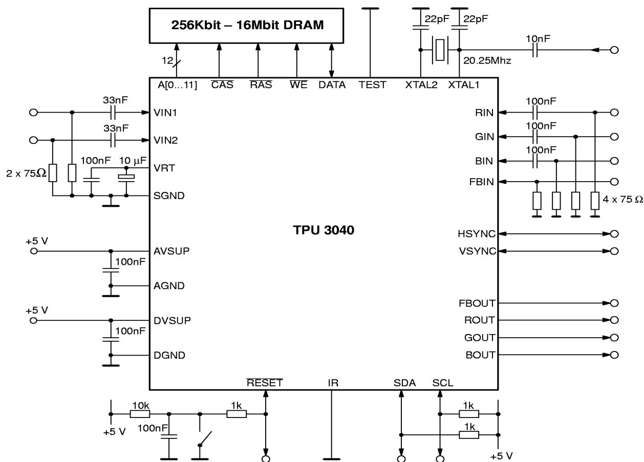
Fig. 5-1: TPU 3040 Application with DRAM
