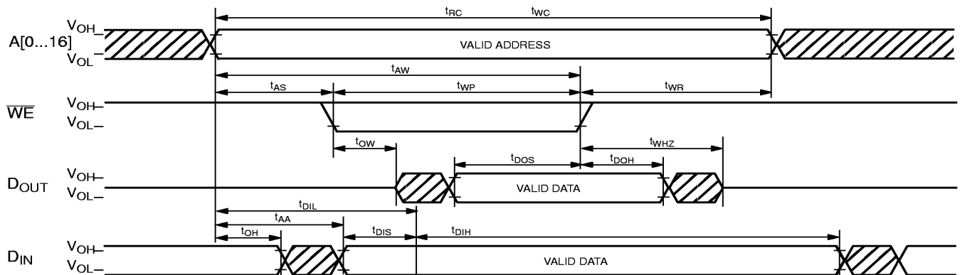
Fig. 3–18: SRAM mode waveforms
