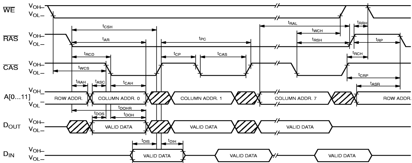
Fig. 3-17: DRAM page mode waveforms
