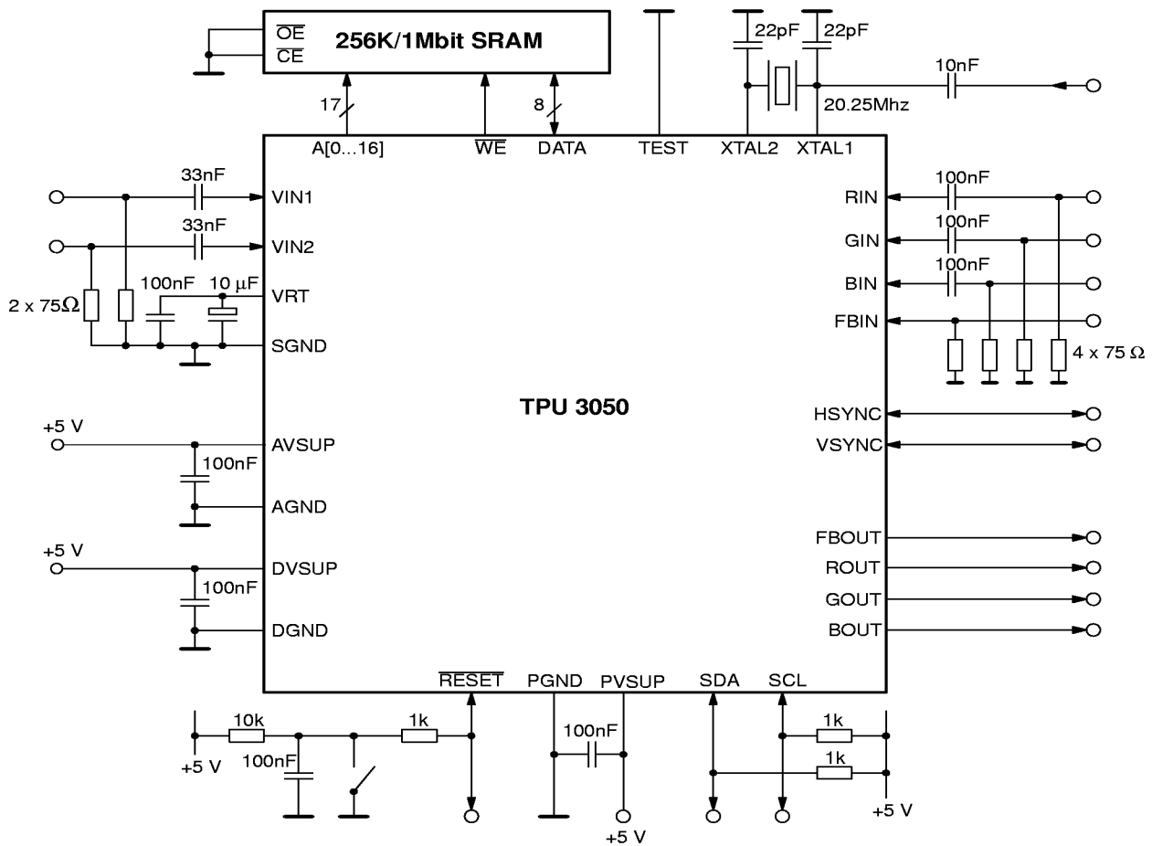
Fig. 5–2: TPU 3050 Application with SRAM
