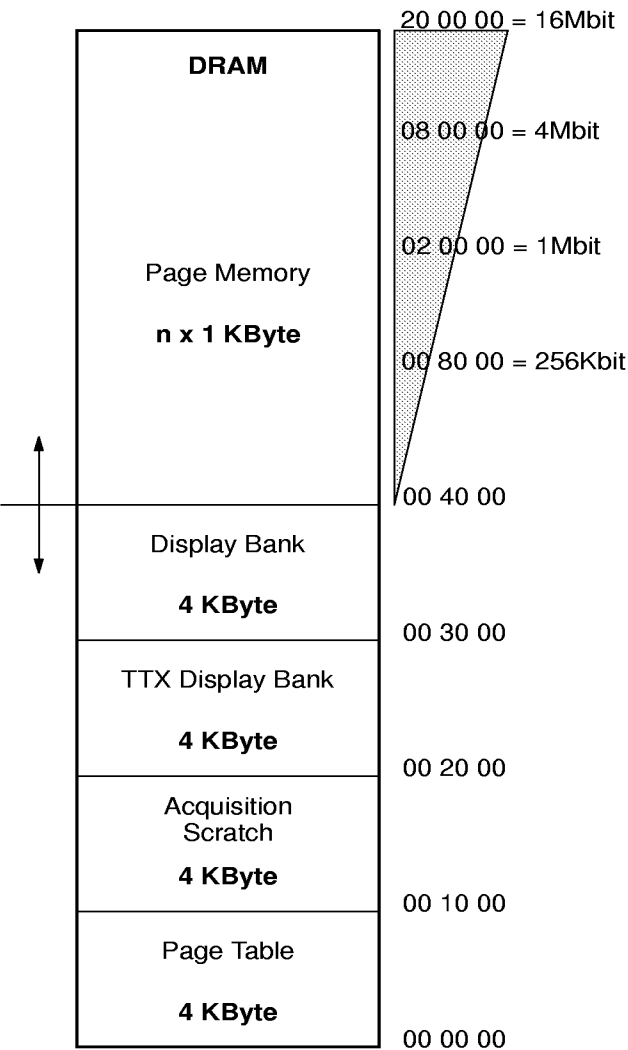
Fig. 4–8: Memory Organization
