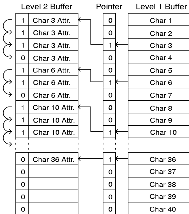
Fig. 2-2: Stack Row Buffer
