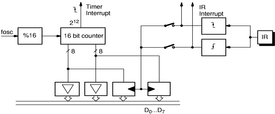
Fig. 2–5: Timer Structure
