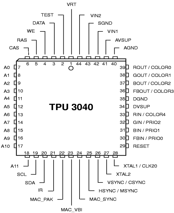
Fig. 3-6: TPU 3040 in 44-pin PLCC package
