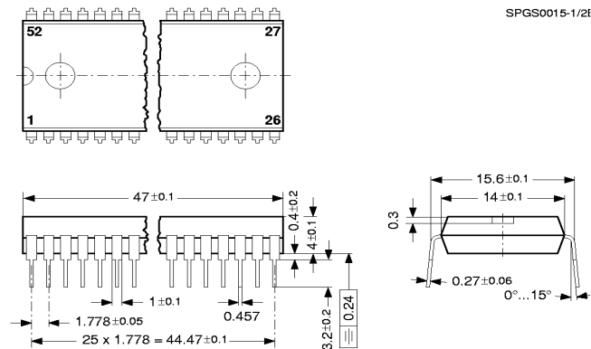
Fig. 3-2: 52-Pin Plastic Shrink Dual-Inline Package (PSDIP52) Weight approximately 5.5 g Dimensions in mm
