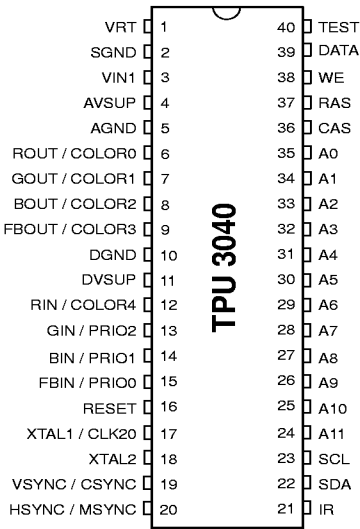
Fig. 3-4: TPU 3040 in 40-pin PDIP package
