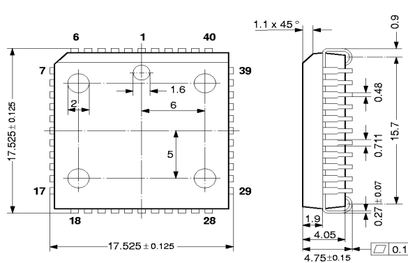
Fig. 3-3: 44-Pin Plastic Leaded Chip Carrier Package (PLCC44) Weight approximately 2.5 g Dimensions in mm
