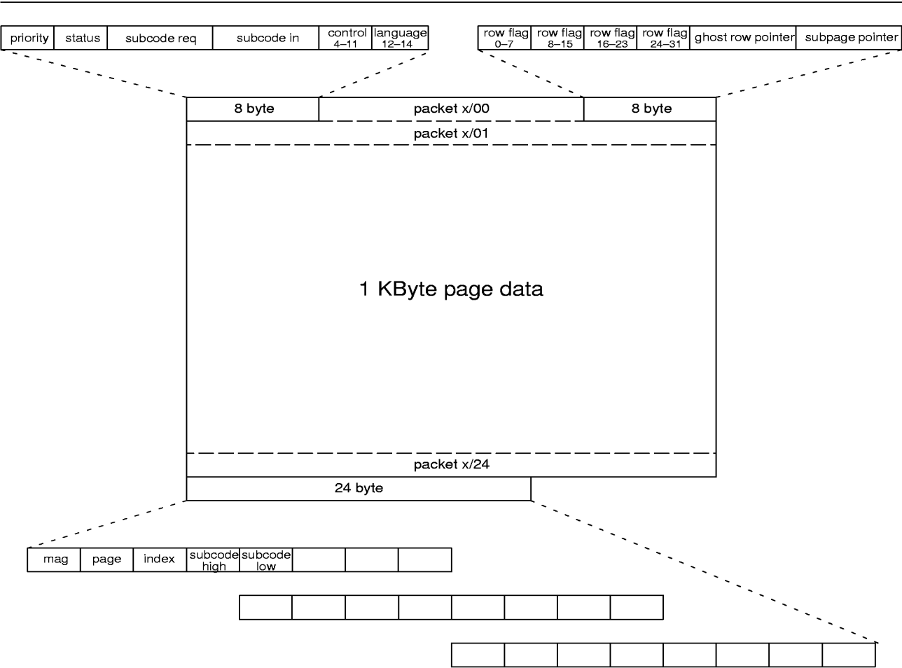
Fig. 4-9: Page Format
