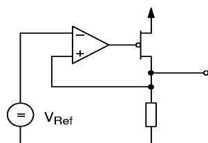
Fig. 3-7: Supply Pin 1
