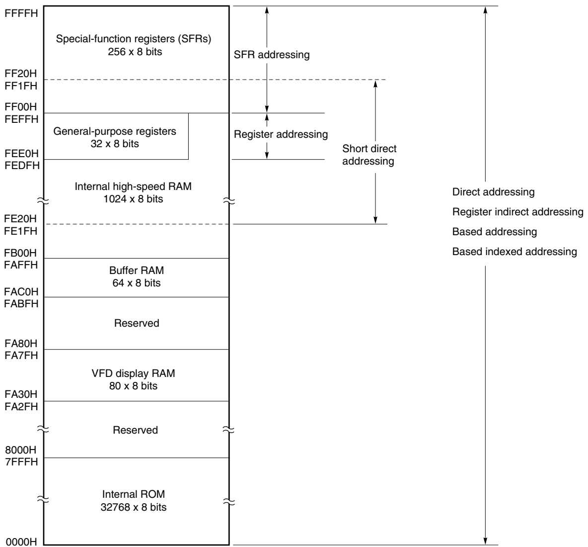
Figure 3-6. Data Memory Addressing ( \mu PD780204 and \mu PD780204A)
