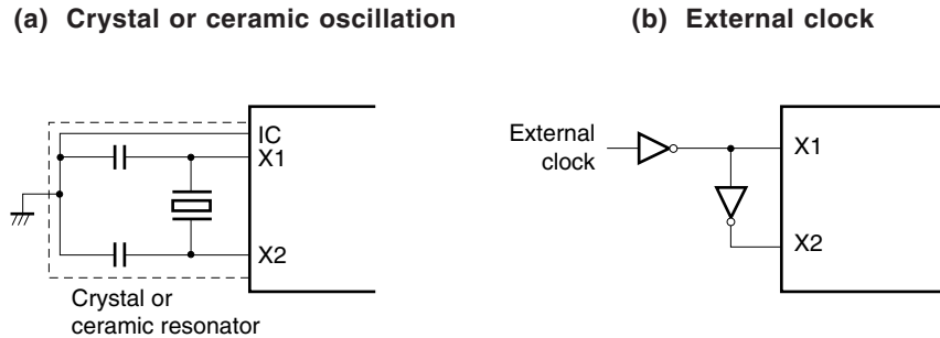
Figure 5-6. External Circuit of Main System Clock Oscillator
