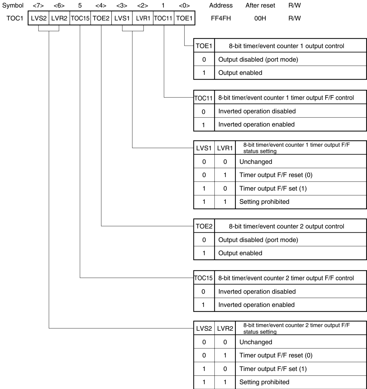
Figure 7-6. Format of 8-Bit Timer Output Control Register
