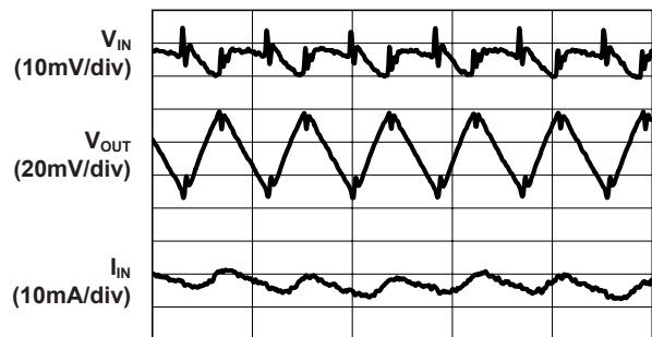
Output Ripple Voltage ( I_{OUT} = 100mA @ V_{IN} = 3.5V )
