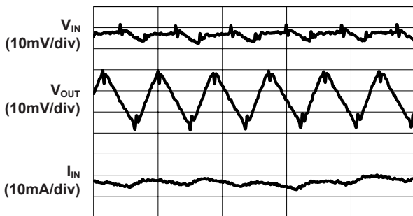
Output Ripple Voltage ( I_{OUT} = 50mA @ V_{IN} = 3.5V )
