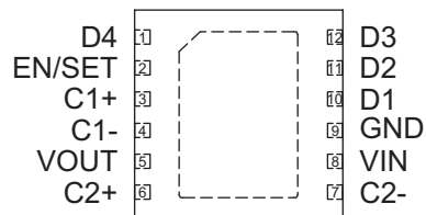
TDFN33-12/STDFN33-12 (Top View)
