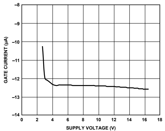
Figure 10. GATE Current (up) vs. Supply Voltage
