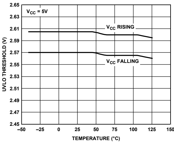
Figure 7. UVLO Threshold vs. Temperature
