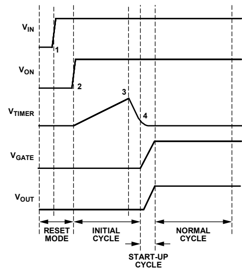
Figure 30. Power-Up Timing
