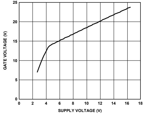
Figure 8. GATE Voltage vs. Supply Voltage
