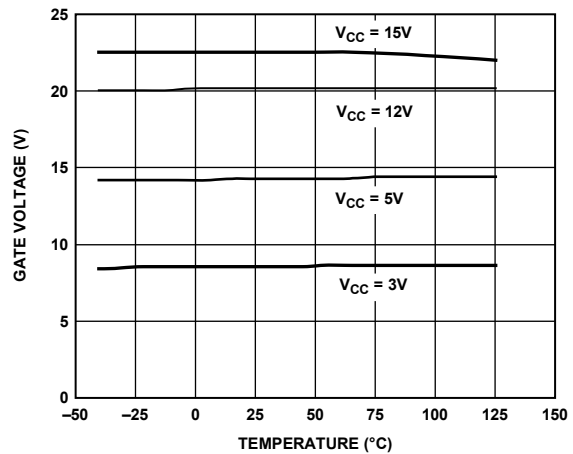
Figure 9. GATE Voltage vs. Temperature
