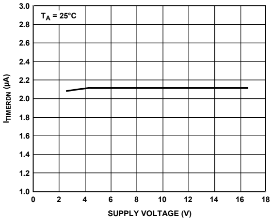
Figure 18. I_TIMERDN (in Cool-Off Cycle) vs. Supply Voltage
