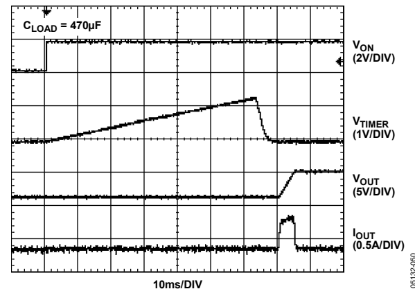
Figure 2. Start-Up Sequence
