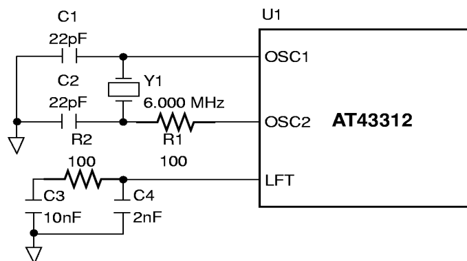
Figure 4. Oscillator and PLL Connections
