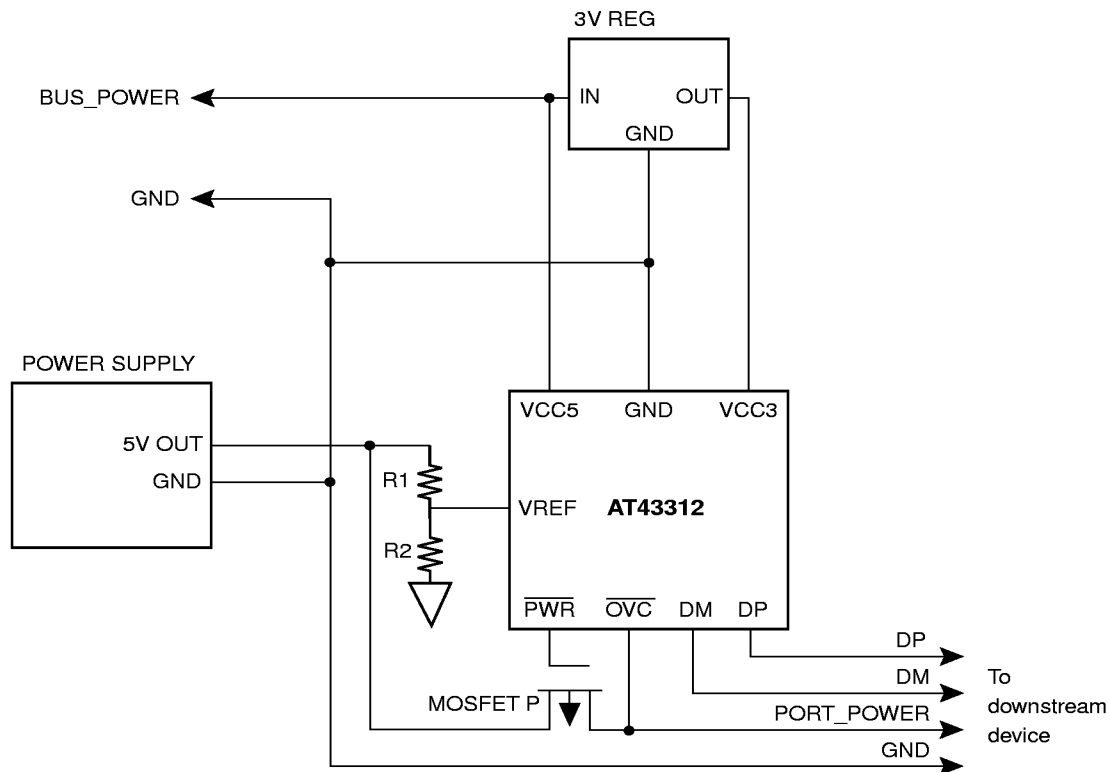
Figure 2. Self-Powered Hub Power Supply
