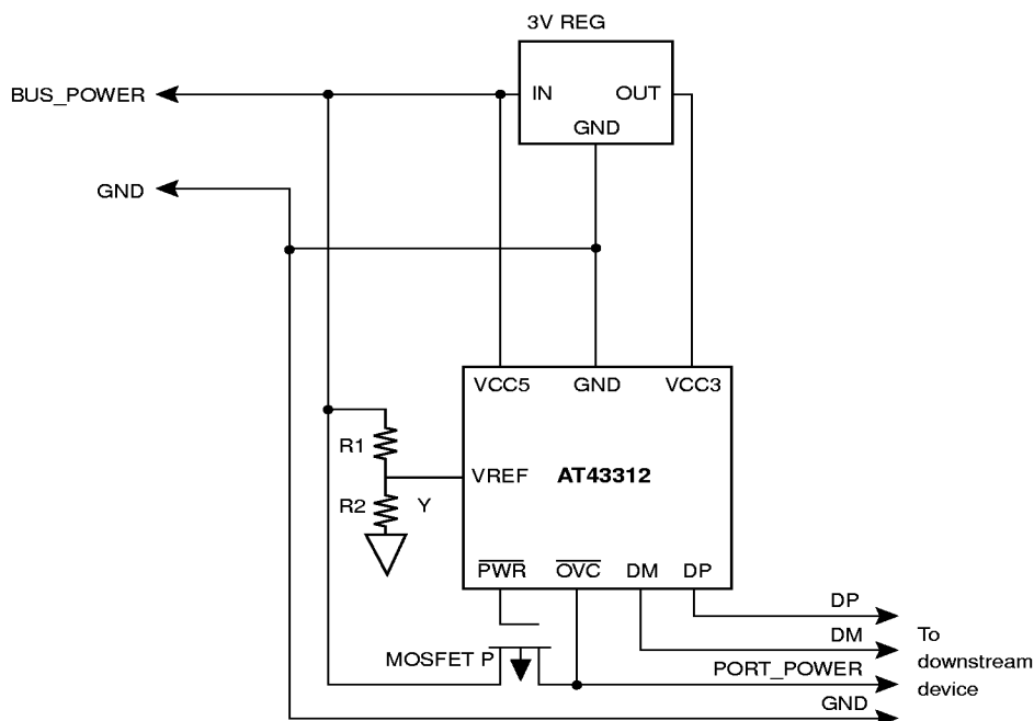
Figure 3. Bus-Powered Hub Power Supply
