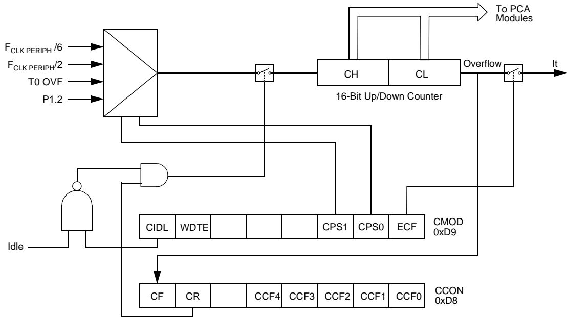
Figure 8. PCA Timer/Counter
