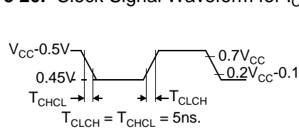
Figure 26. Clock Signal Waveform for I_{CC} Tests in Active and Idle Modes
