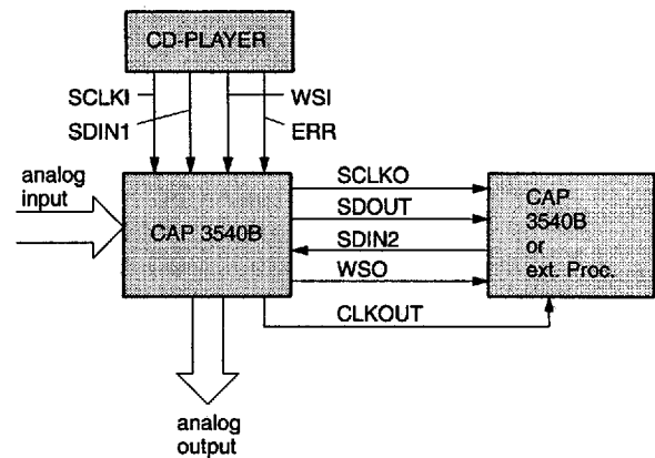
Fig. 2-12: System configuration
