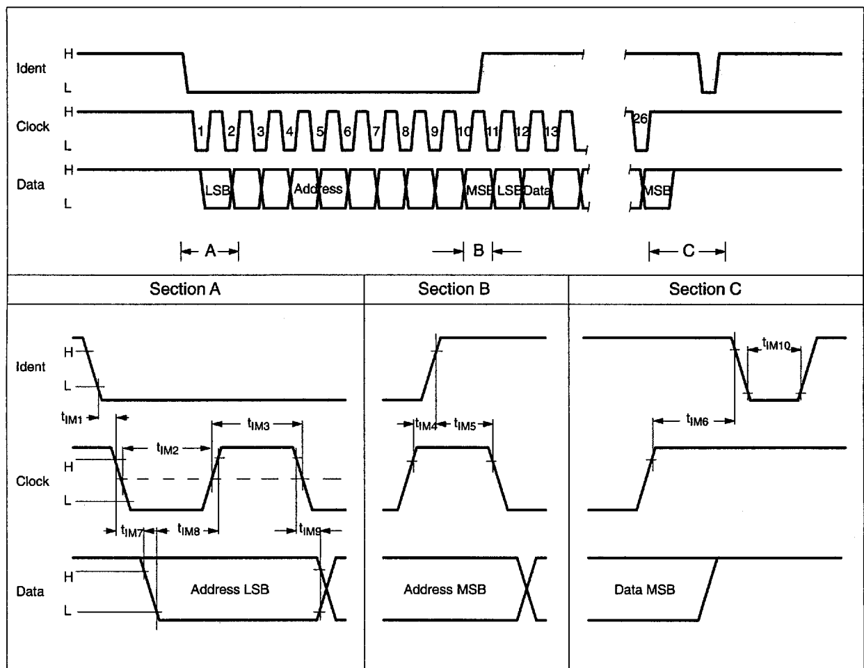
Fig. 2-16: IM-Bus waveforms
