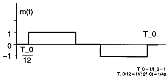
Fig. 2-4: Difference channel mixing signal
