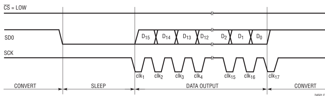
Figure 12. 2-Wire, Idle-High (CPOL = 1) Serial Clock, Operation Example
