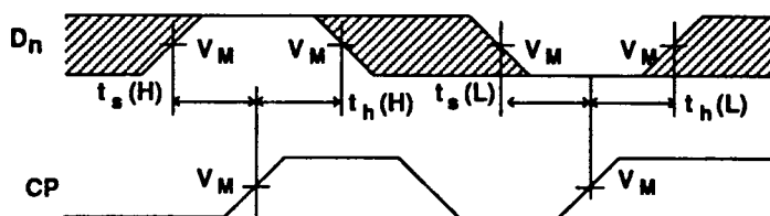
Waveform 3. Data Setup And Hold Times
