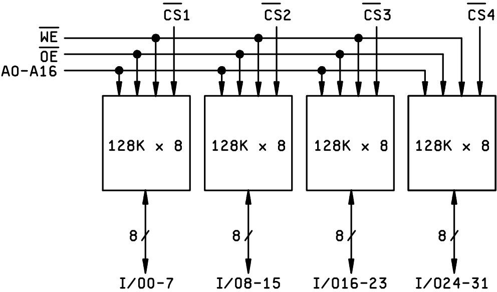
FIGURE 7. Block diagrams .
