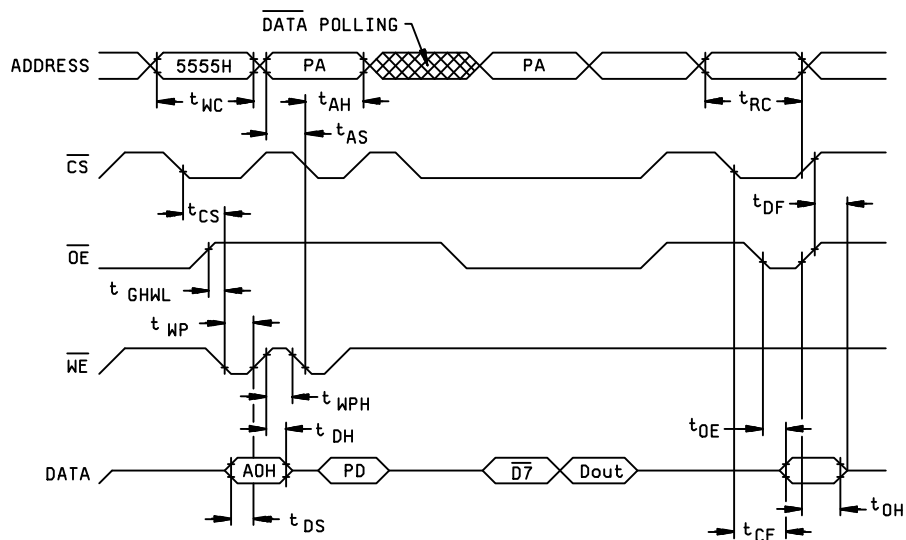
FIGURE 5. Write/Erase/Program operations, \overline{WE} controlled.
