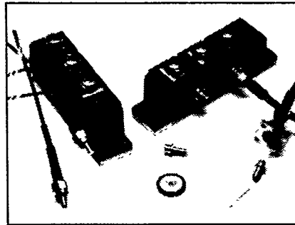
CDL3 — 60 Dual SCR Light-Triggered POW-R-BLOK™ Module 60 Amperes/100-1400 Volts
