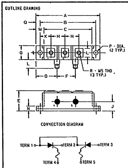
CDL3 — 60 Dual SCR Light-Triggered POW-R-BLOK™ Module 60 Amperes/100-1400 Volts
