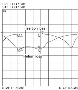
Insertion Loss and Return Loss
