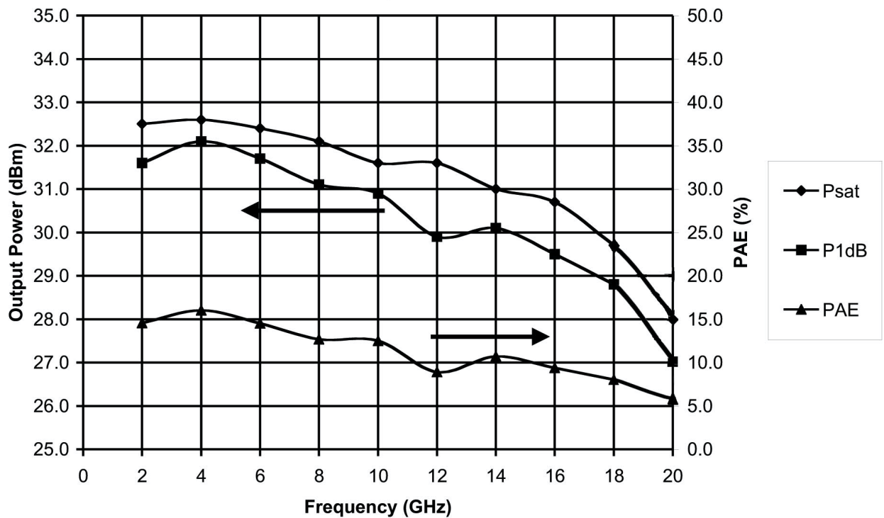
CMM0016-BD Typical Measured Data (connectorized test fixture) Vdd=12V, Idd=700mA
