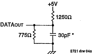
Figure 1. Output Load
