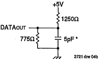
Figure 2. Output Load (for tLZ, tHZ, tWZ, tOW)
