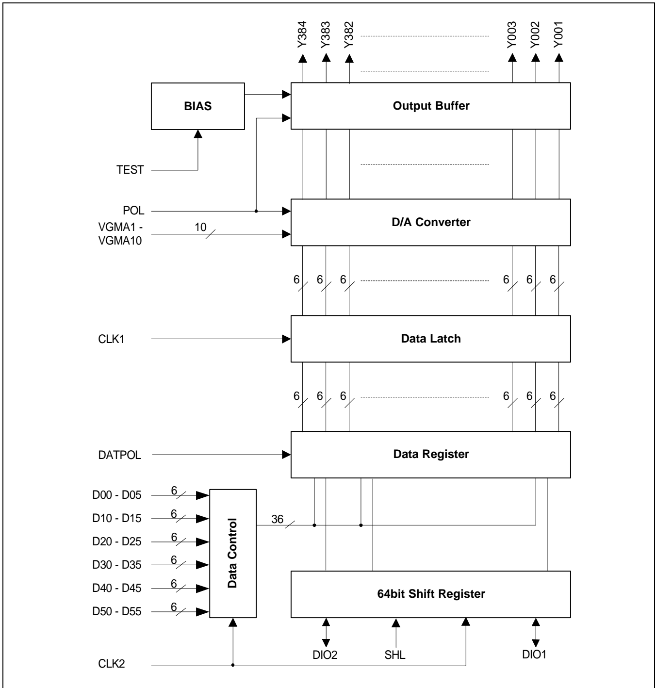
Figure 1. KS0672 Block Diagram
