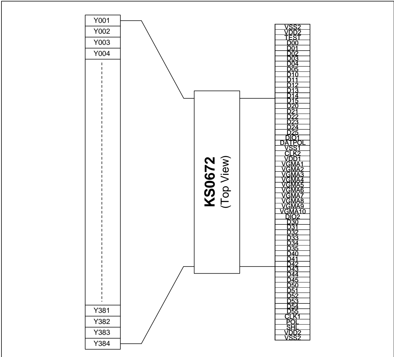
Figure 2. KS0672 Pin Assignments
