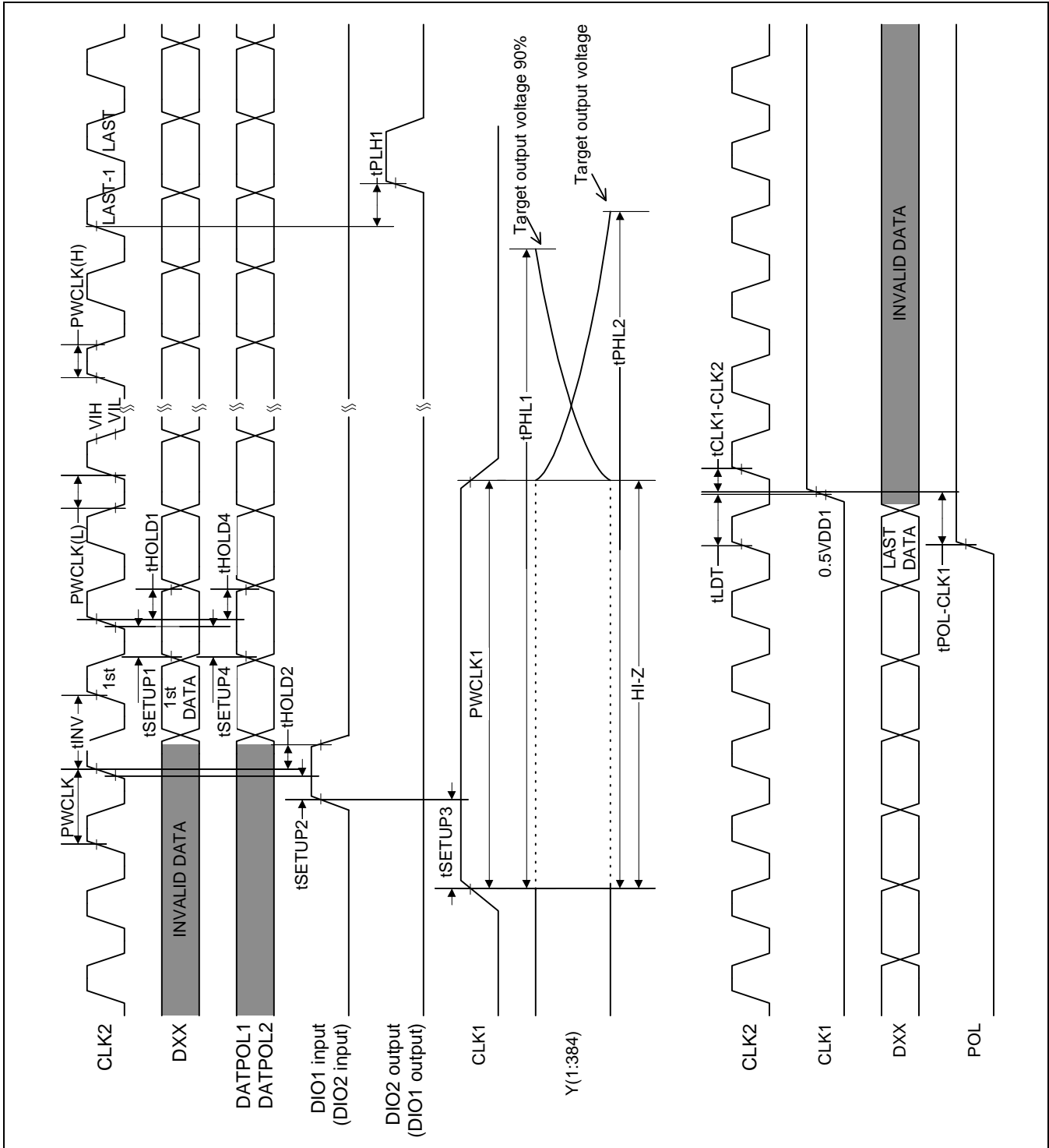
Figure 6. Waveforms
