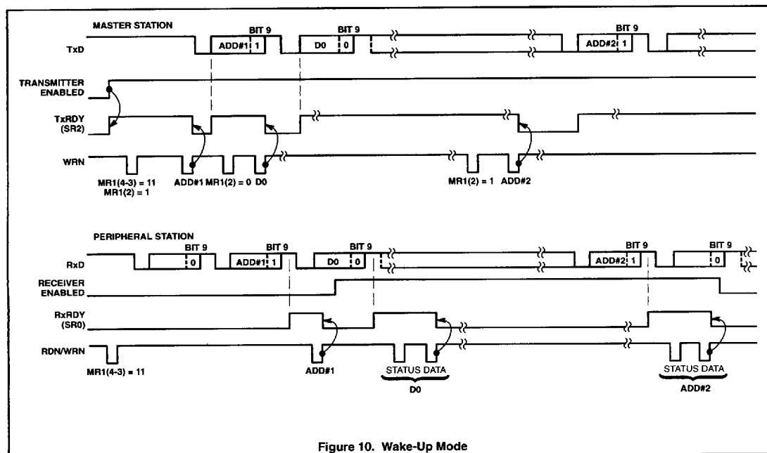
Figure 10. Wake-Up Mode
