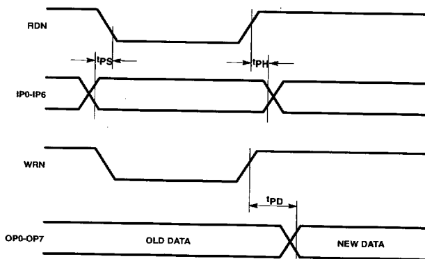
Figure 3. Port Timing
