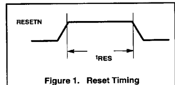
Figure 1. Reset Timing
