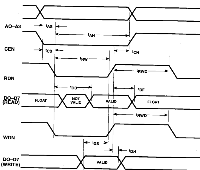
Figure 2. Bus Timing
