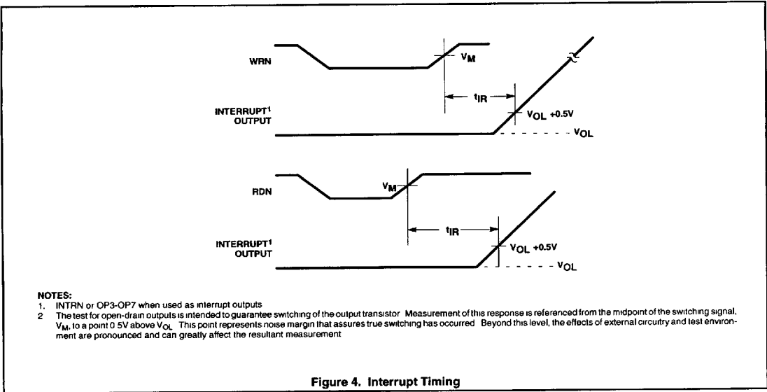
Figure 4. Interrupt Timing
