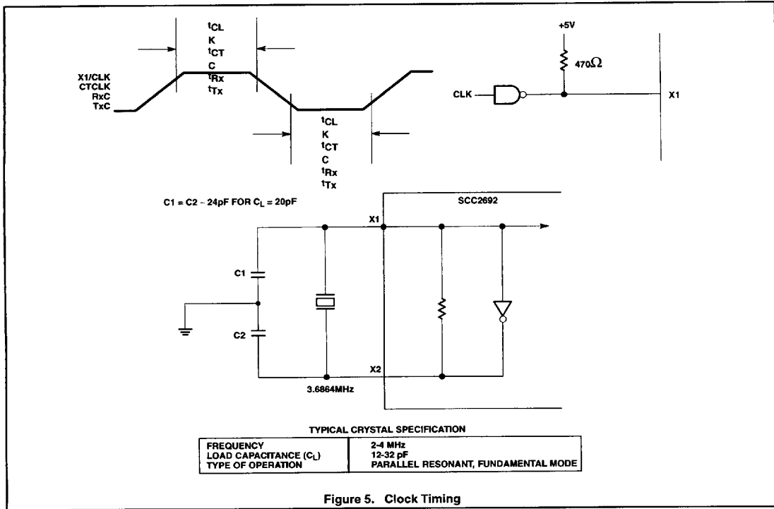
Figure 5. Clock Timing
