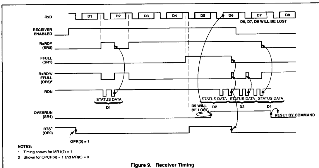
Figure 9. Receiver Timing
