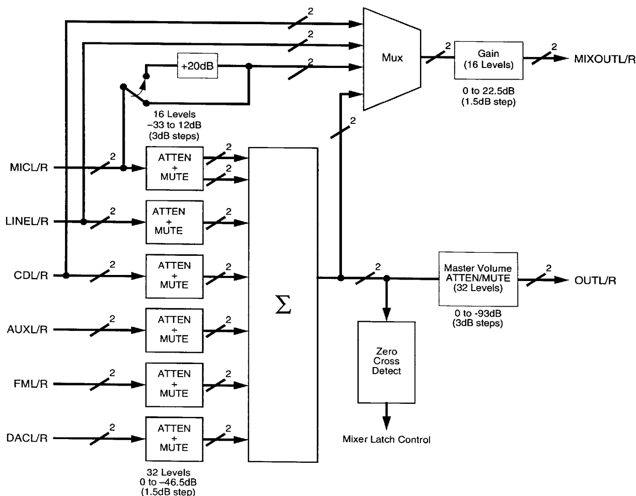
Figure 4-2 Mixer Block Diagram
