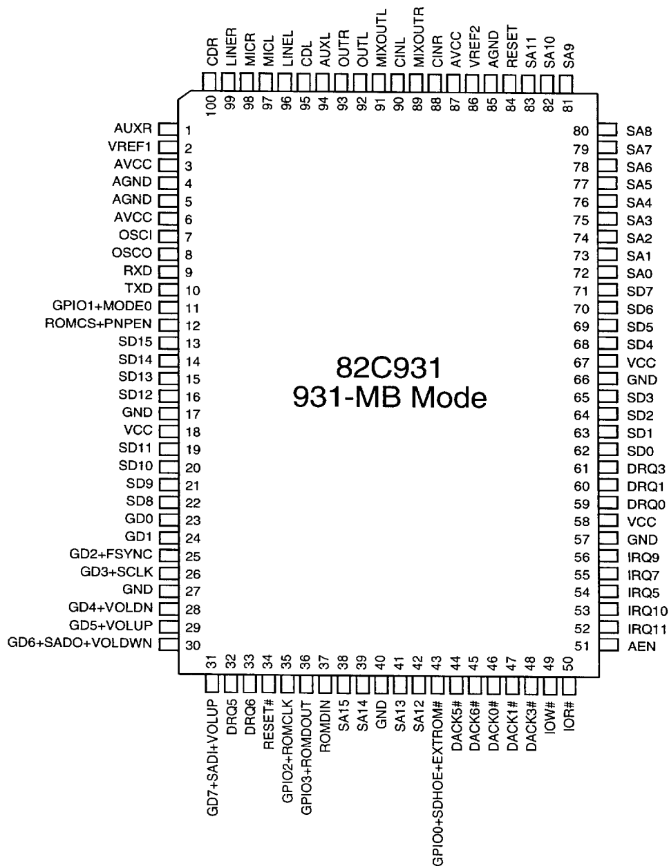
Figure 3-1 931-MB Mode PQFP Pin Diagram *
