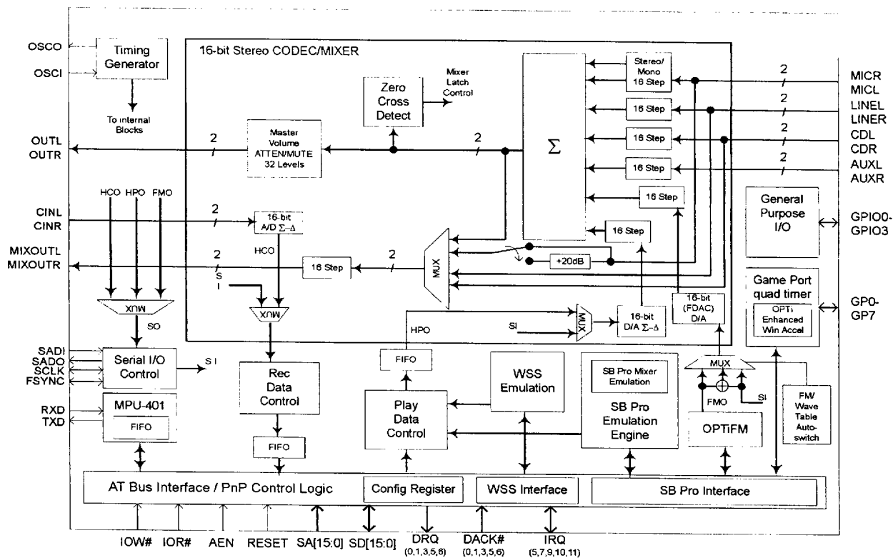
Figure 2-2 Data Flow Block Diagram
