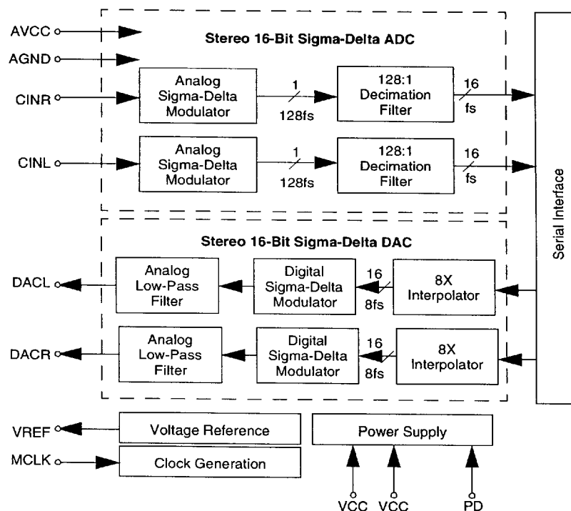
Figure 4-1 Functional Block Diagram
