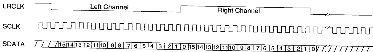
Figure 4-3 I 2 S Format
