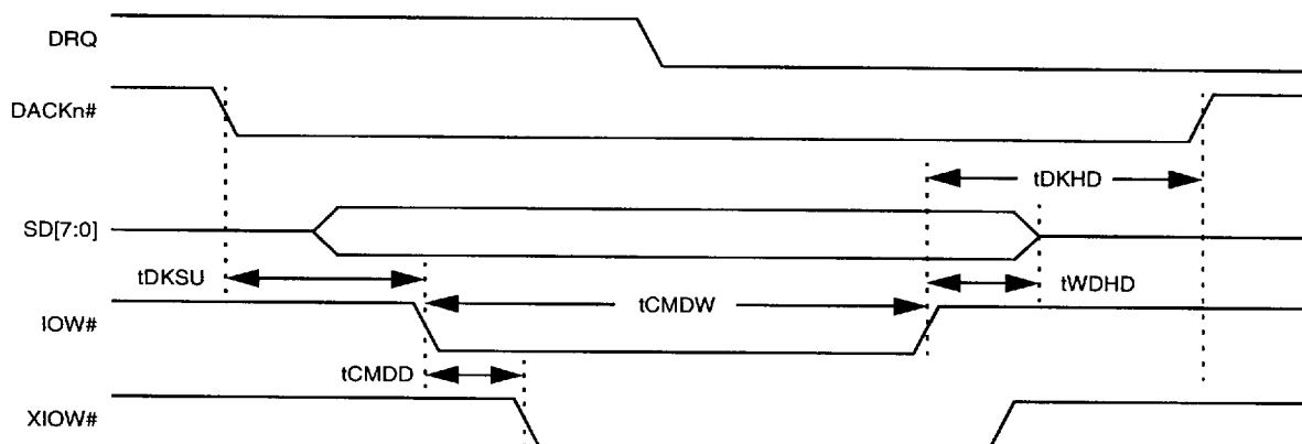
Figure 6-4 DMA Write/Playback Cycle
