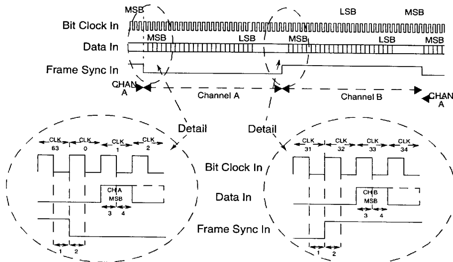
Figure 4-4 General Purpose Serial Port, Timing Relationships
