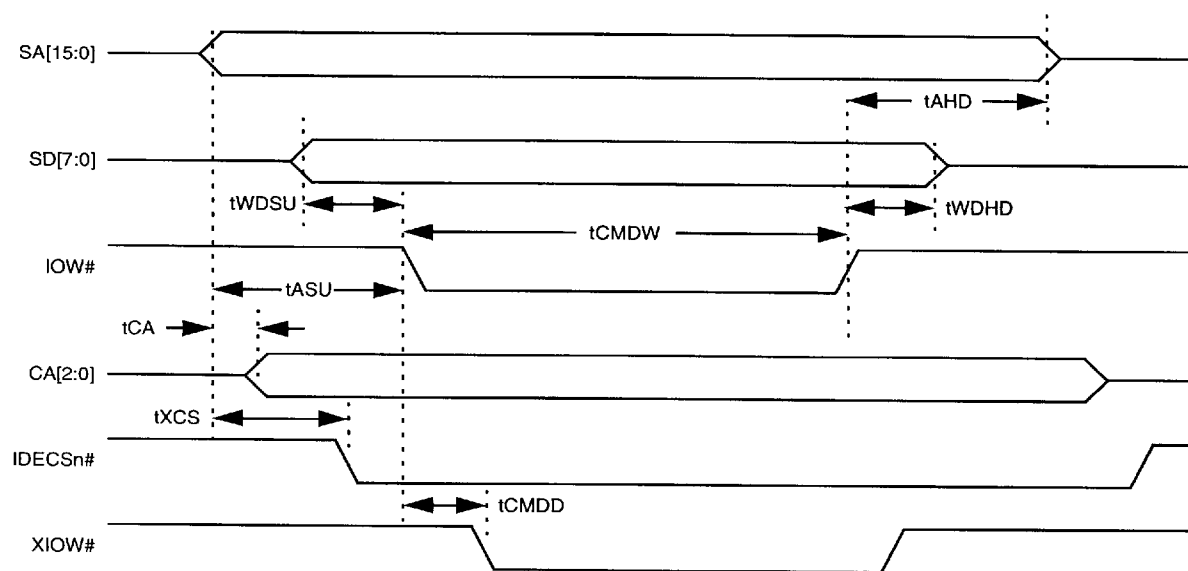
Figure 6-3 CD-ROM I/O Write Cycle
