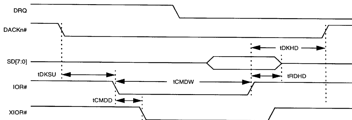
Figure 6-5 DMA Read/Capture Cycle
