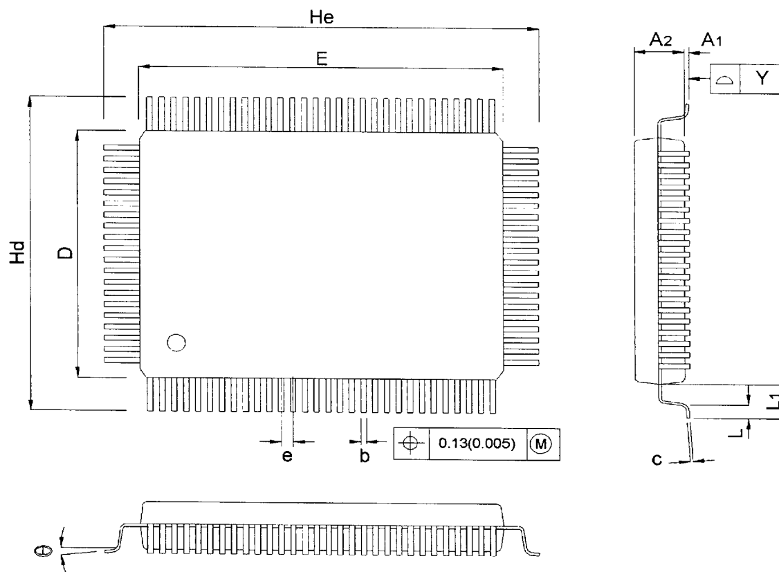
Figure 7-1 100-pin PQFP, Plastic Quad Flat Pack
