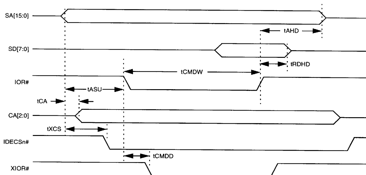
Figure 6-2 CD-ROM I/O Read Cycle
