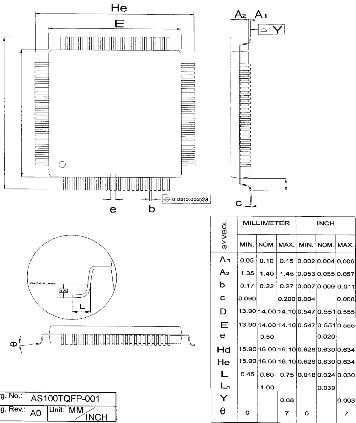
Figure 7-2 100-pin TQFP, Thin Quad Flat Package
