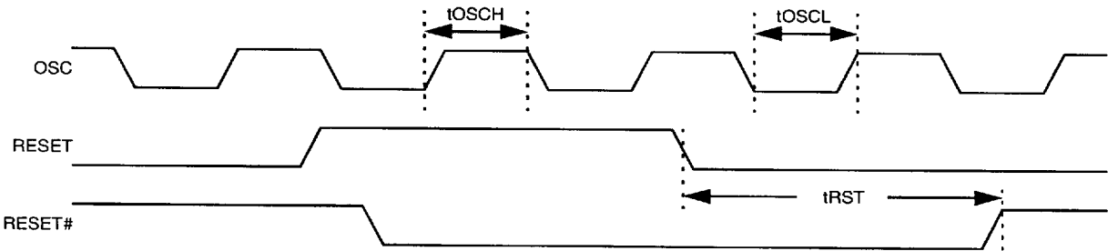
Figure 6-1 RESET and CLK Timing Waveform
