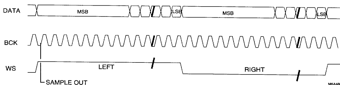
Figure 4-5 Format of Input Signals
