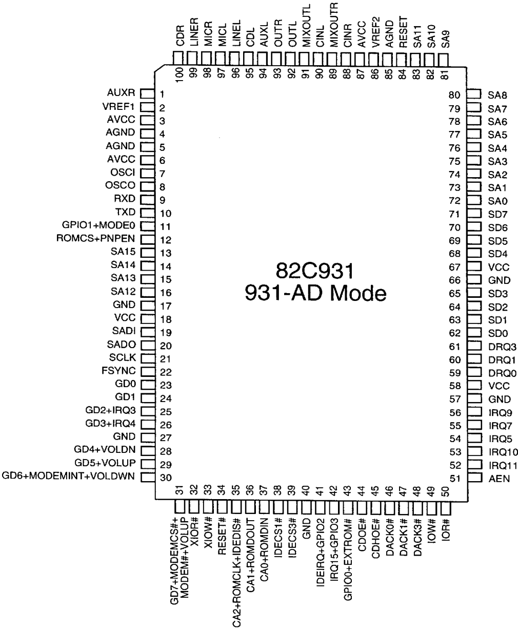
Figure 3-2 931-AD Mode PQFP Pin Diagram *
