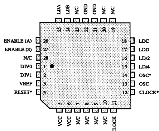
A 28-pin Plastic J-Lead (PLCC) Package
