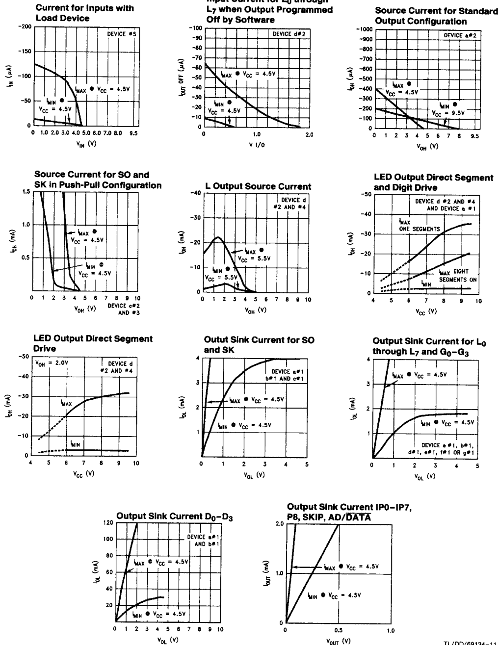
FIGURE 7. I/O Characteristics
