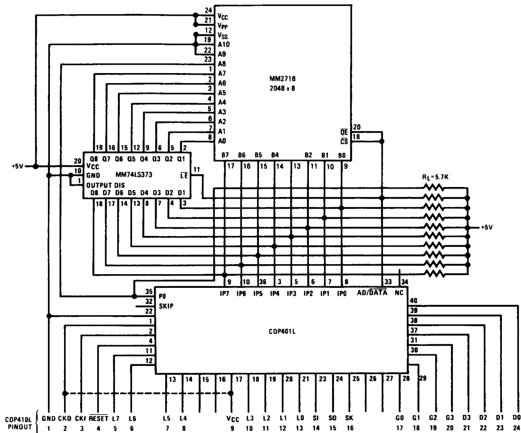
FIGURE 8. COP401L Used to Emulate a COP410L
