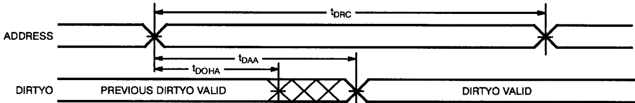
Dirty Read Cycle No. 1 [16, 17]
