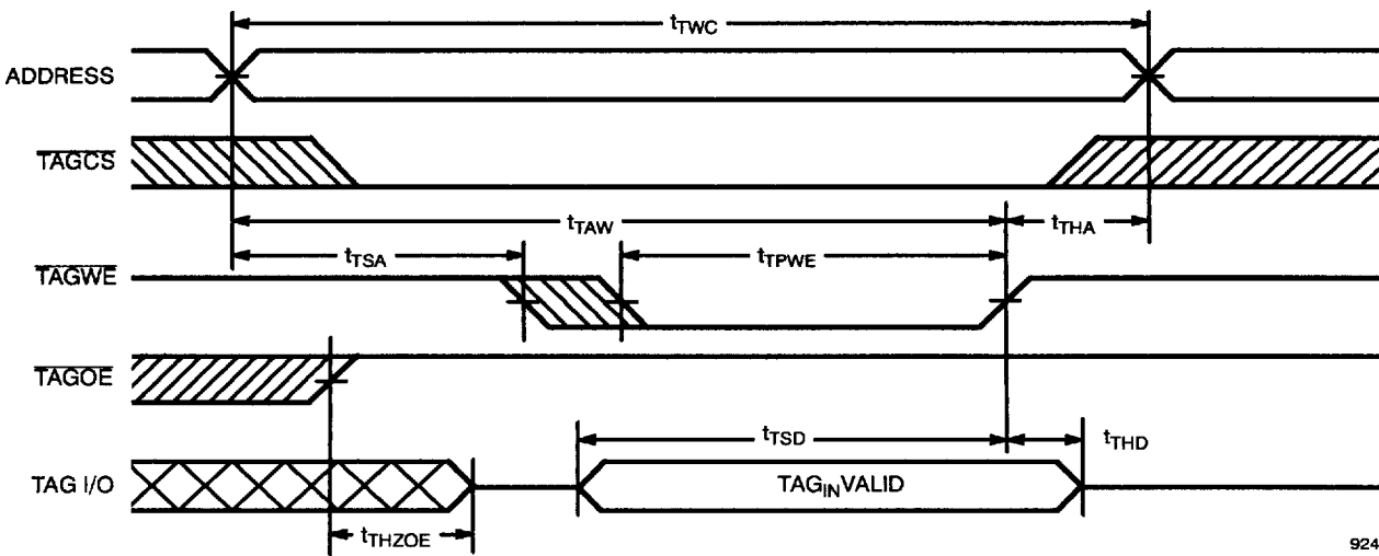
Tag Write Cycle No. 2 (TAGCS Controlled) [13, 14, 15]
