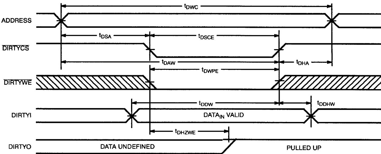
Dirty Write Cycle No. 2 (DIRTYCS Controlled) [19, 20]
