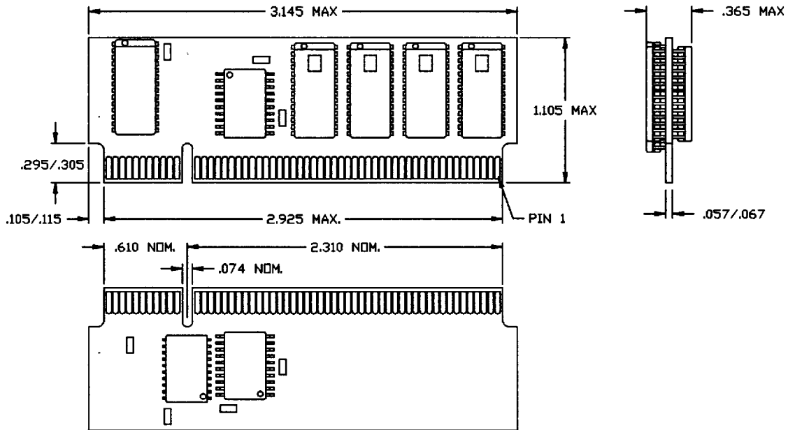
112-Pin Dual-Readout SIMM PB17
