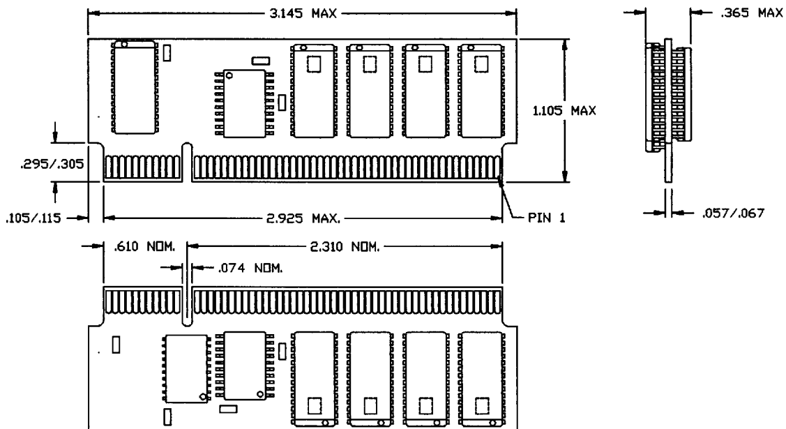
112-Pin Dual-Readout SIMM PB18
