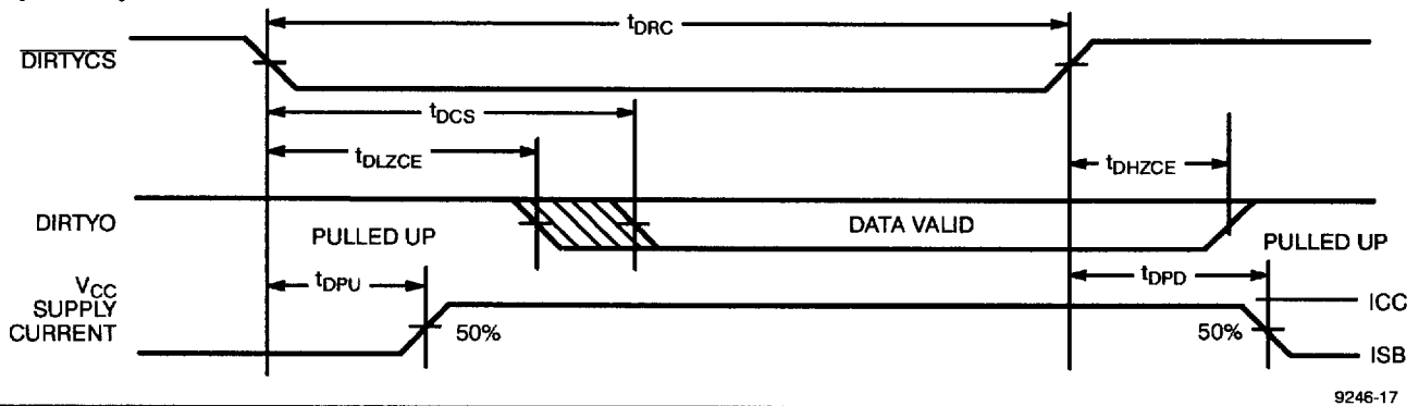
Dirty Read Cycle No. 2 [11, 18]
