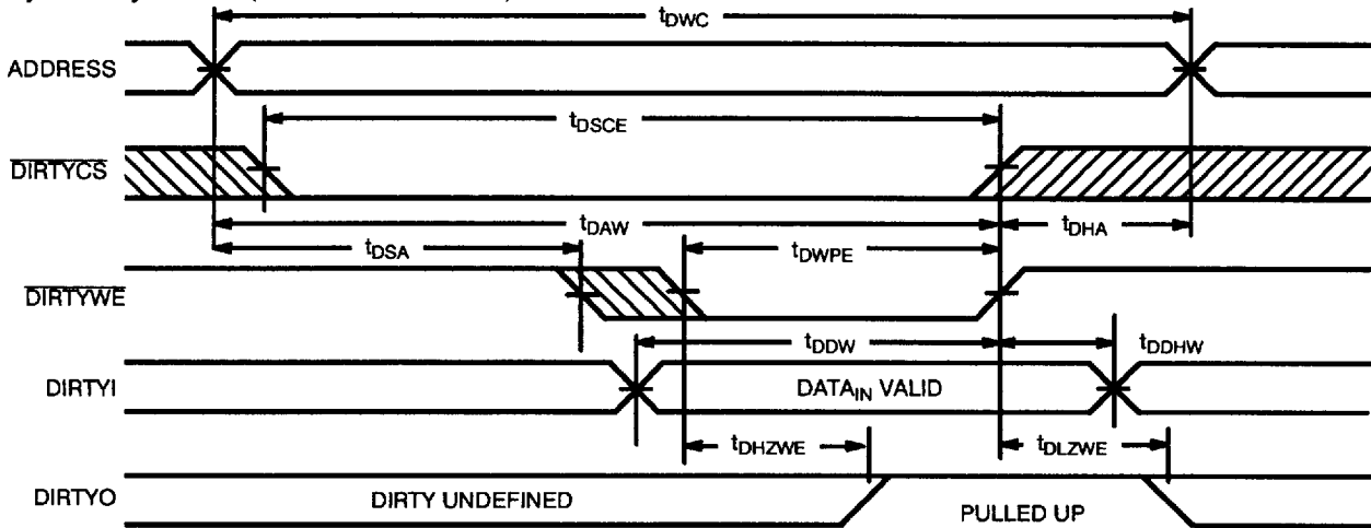
Dirty Write Cycle No. 1 (DIRTYWE Controlled) [19]
