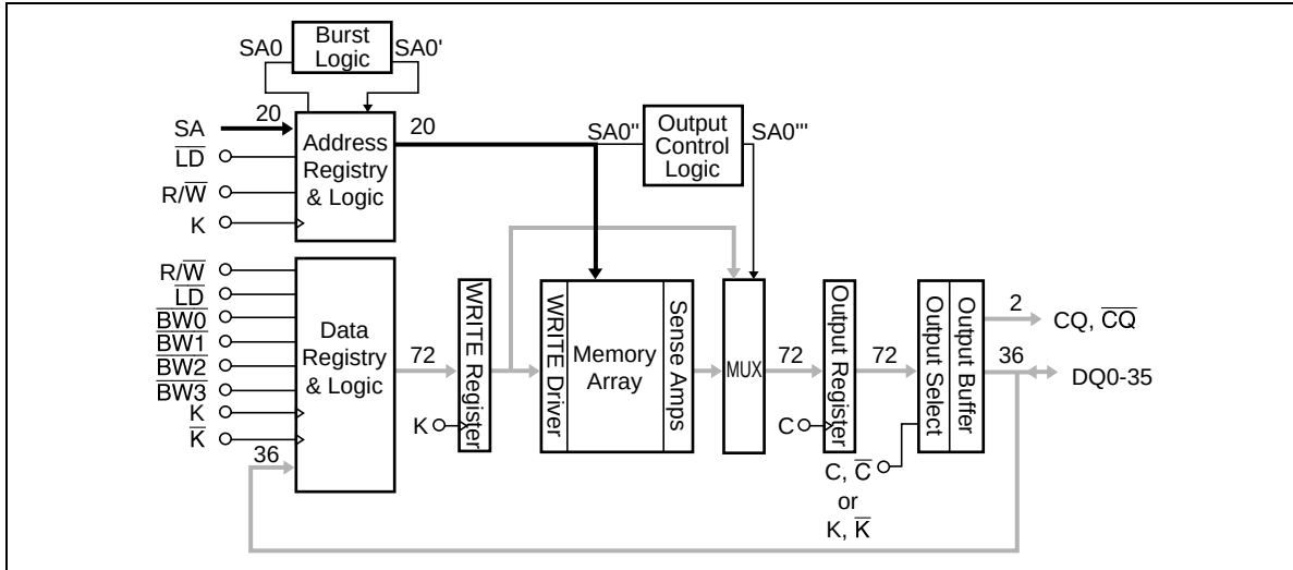
Block Diagram (HM66AEB36102)
