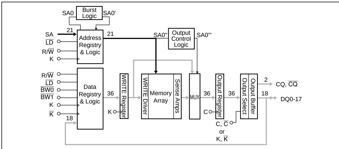
Block Diagram (HM66AEB18202)
