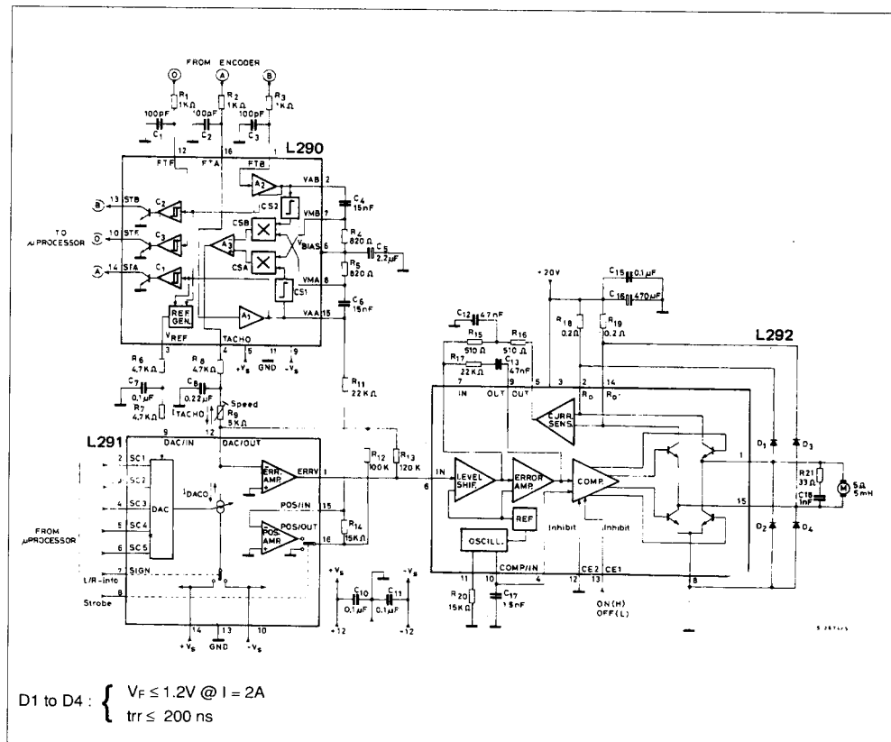
Figure 1 : Complete Application Circuit.
