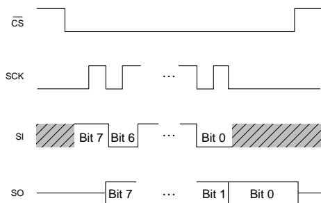
FIGURE 4. SPI Protocol
