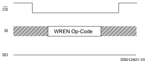
FIGURE 8. Write Enable
