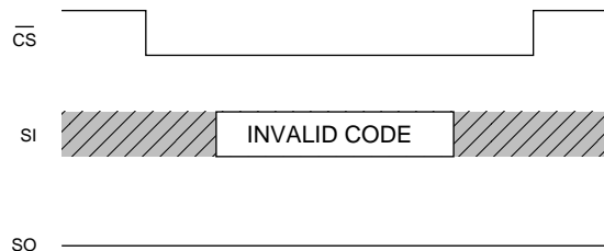
FIGURE 5. Invalid Op-Code
