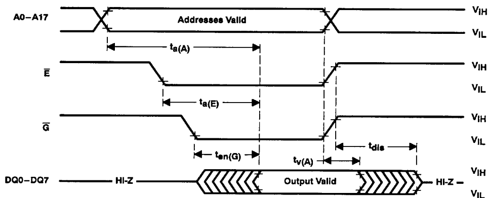
Figure 3. Read-Cycle Timing
