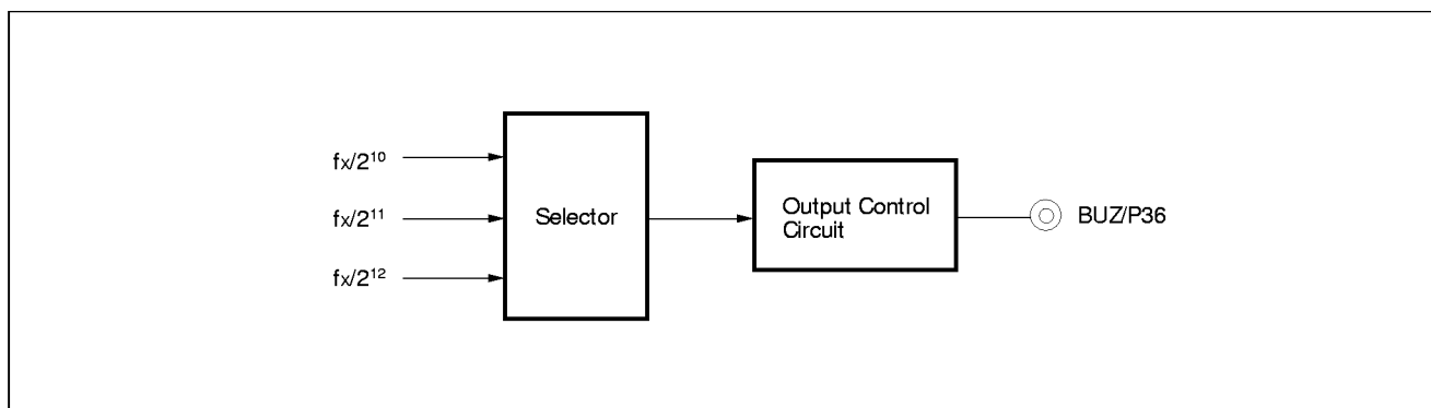
Fig. 5-6 Buzzer Output Control Block Diagram
