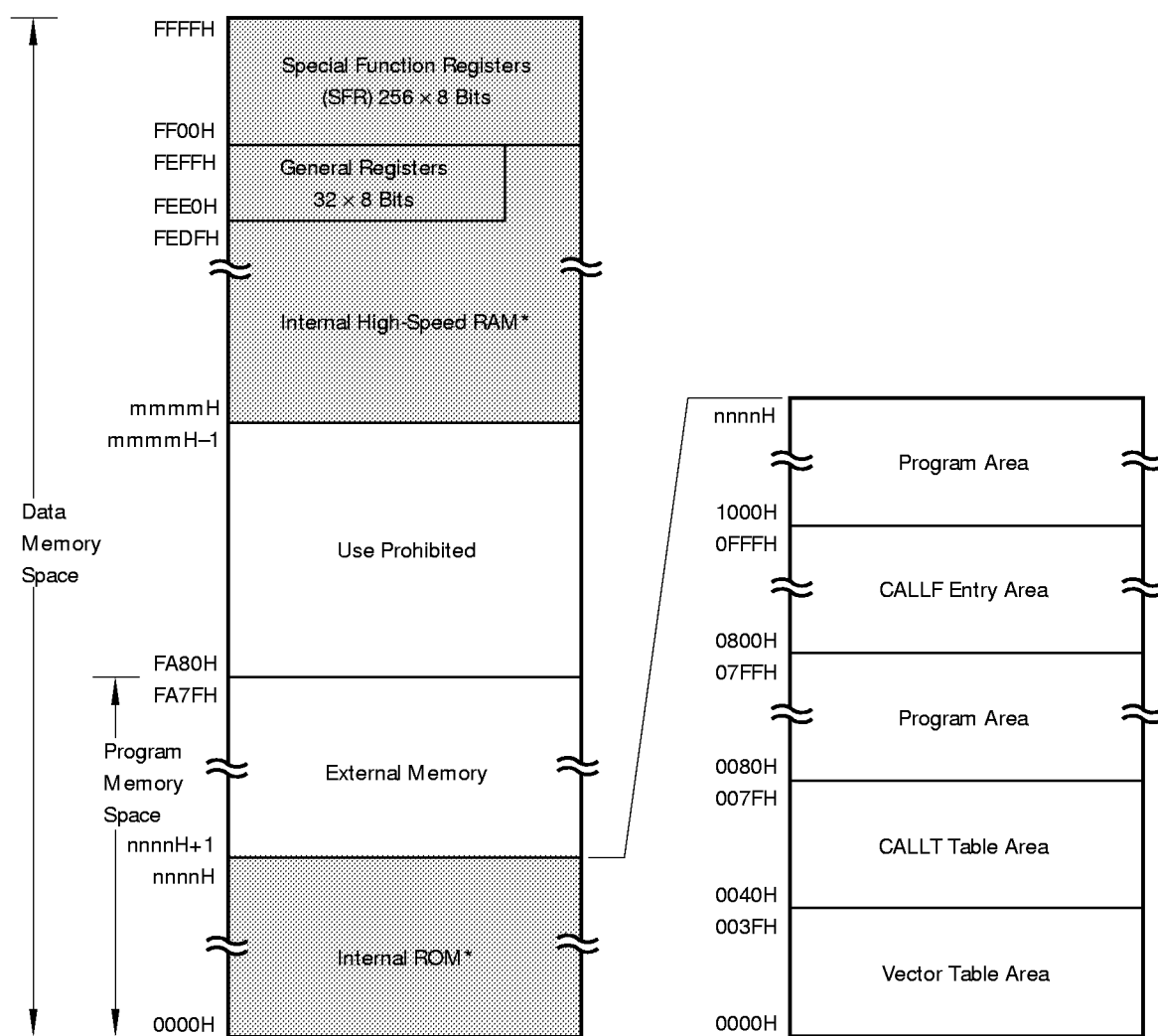
Fig. 4-1 Memory Map
