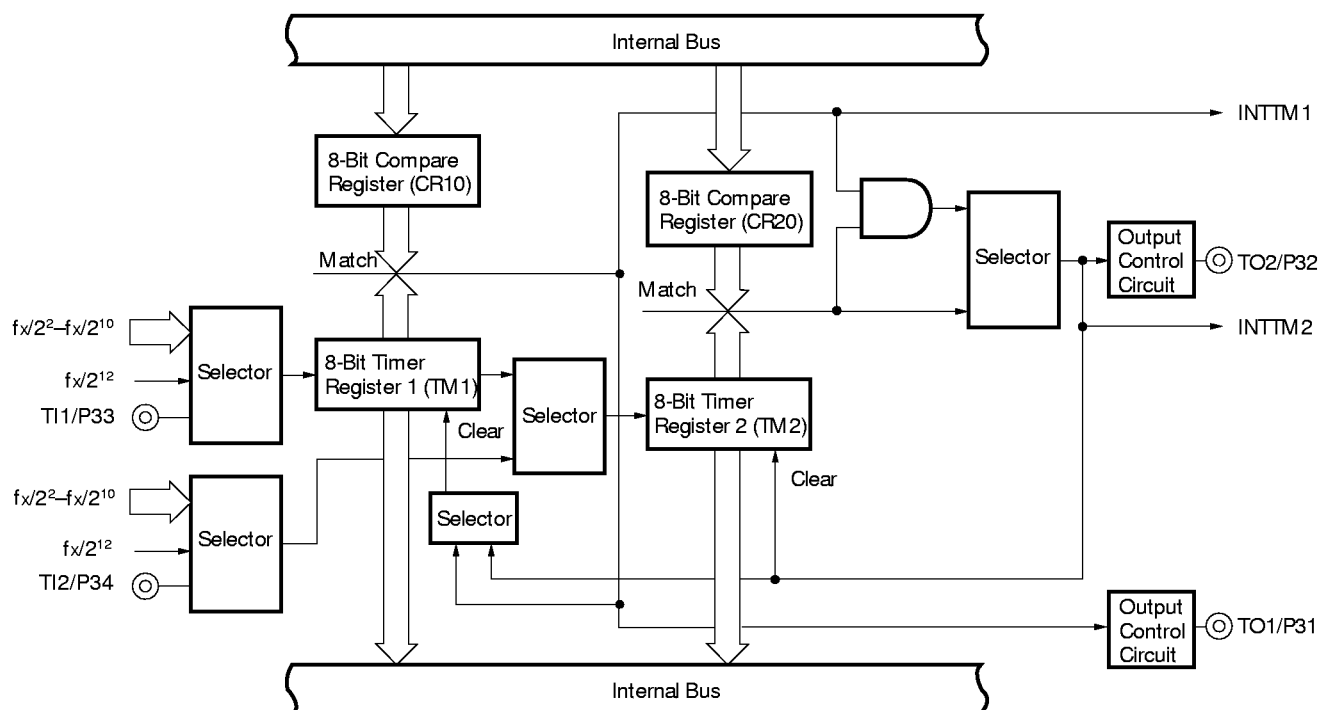
Fig. 5-2 8-bit Timer/ Enent Counter Block Diagram
