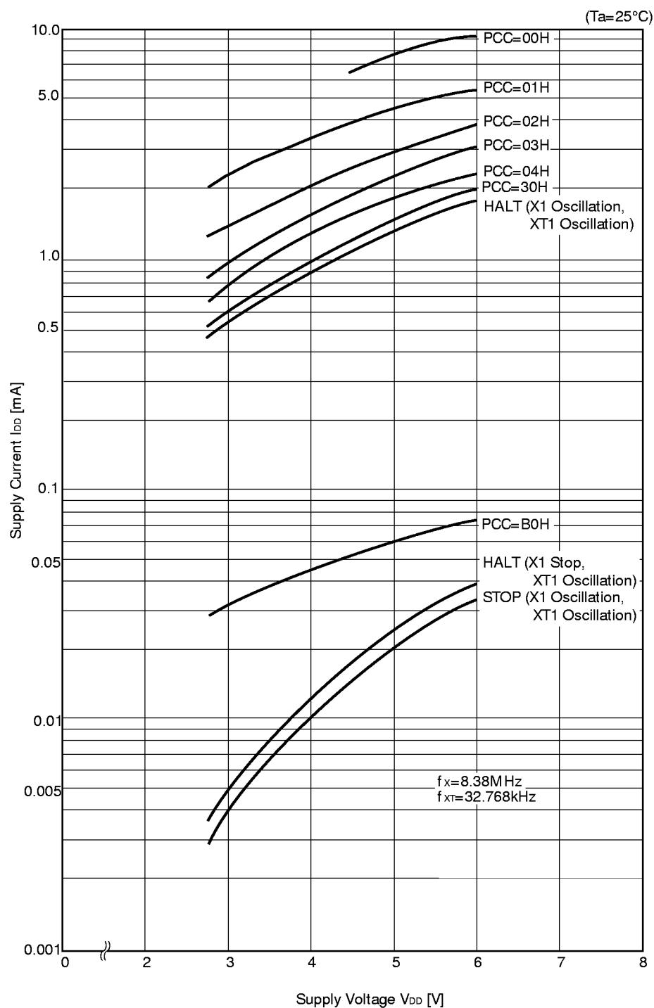
I_{DD} vs V_{DD} (Main System Clock : 8.38 MHz)
