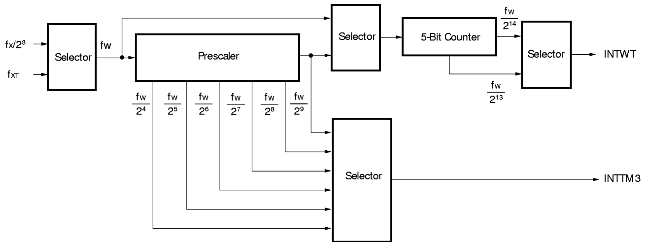
Fig. 5-3 Watch Timer Block Diagram
