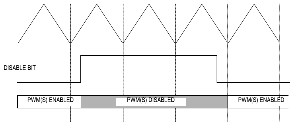
Figure 9-30. PWM Software Disable
