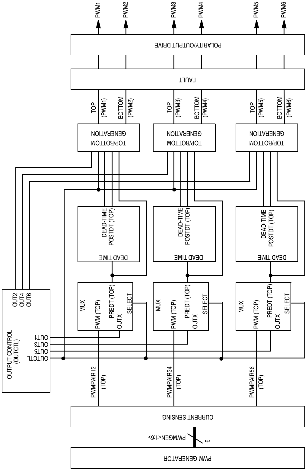
Figure 9-13. Dead-Time Generators
