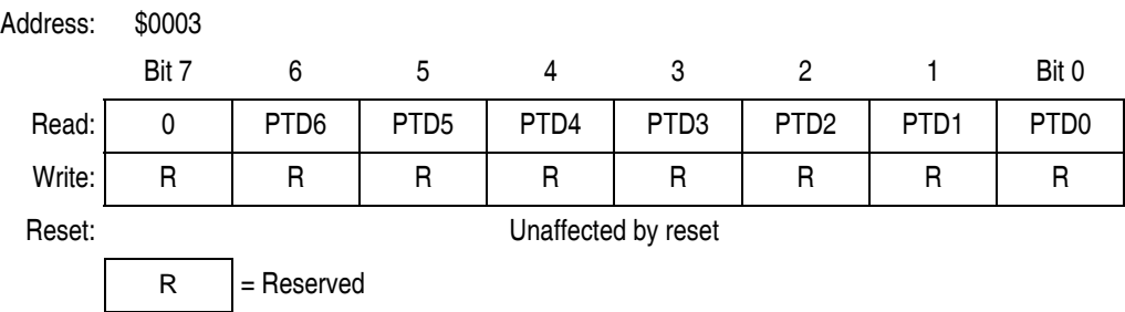
Figure 15-11. Port D Data Register (PTD)
