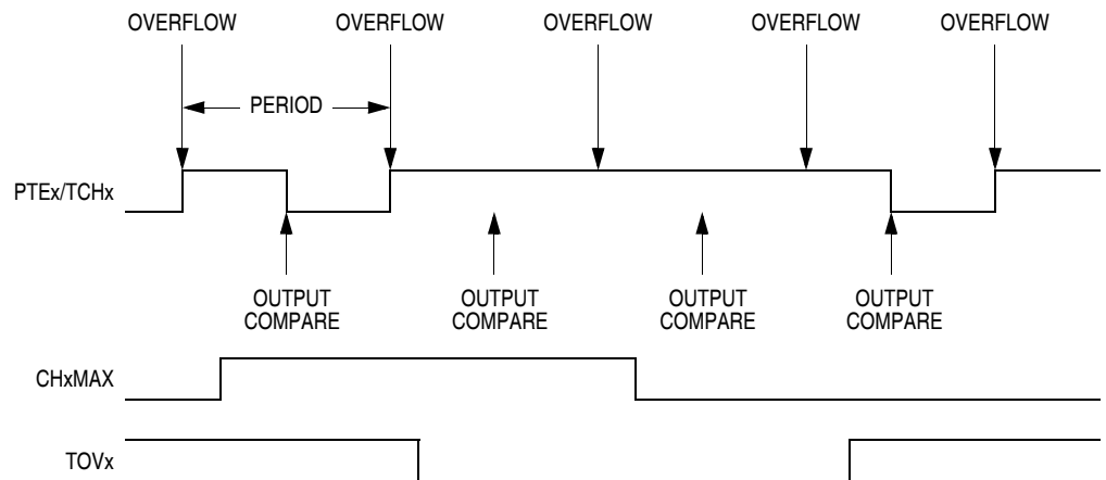
Figure 12-8. CH x MAX Latency
