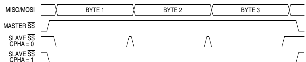
Figure 13-5. CPHA/\overline{SS} Timing
