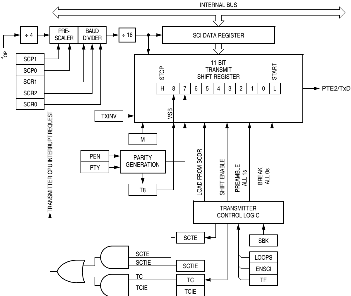
Figure 14-4. SCI Transmitter
