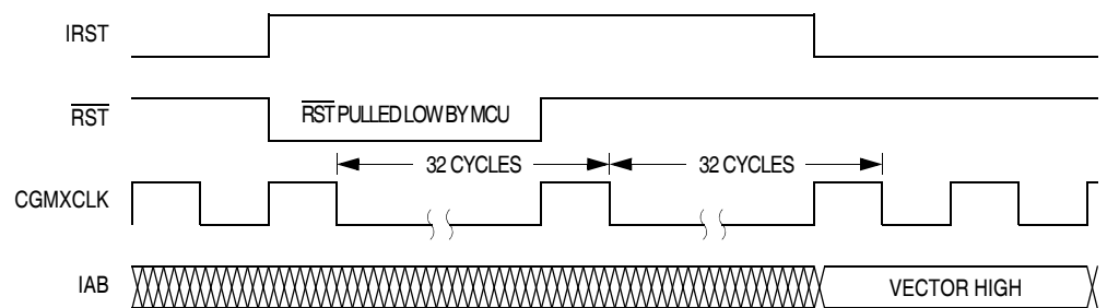
Figure 7-4. Internal Reset Timing
