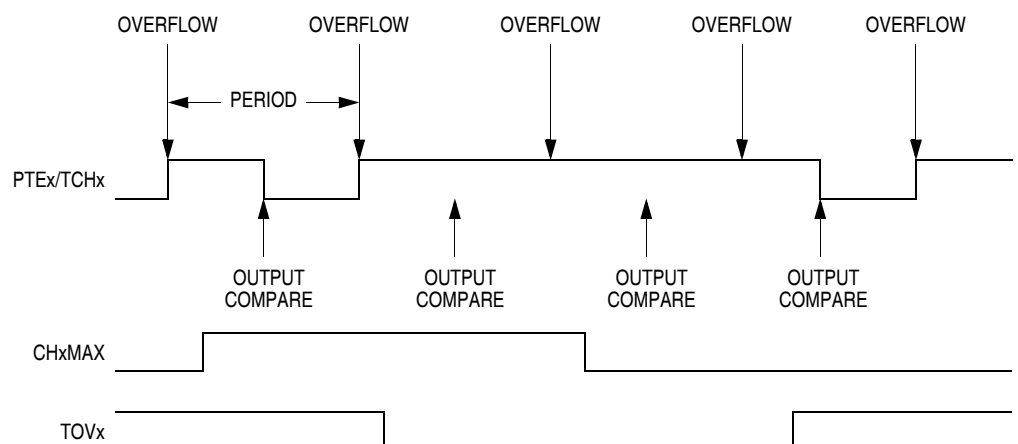
Figure 11-8. CHxMAX Latency
