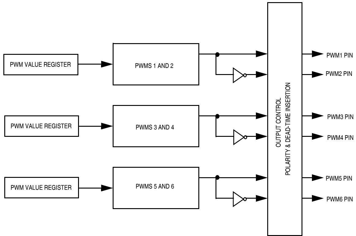
Figure 9-11. Complementary Pairing
