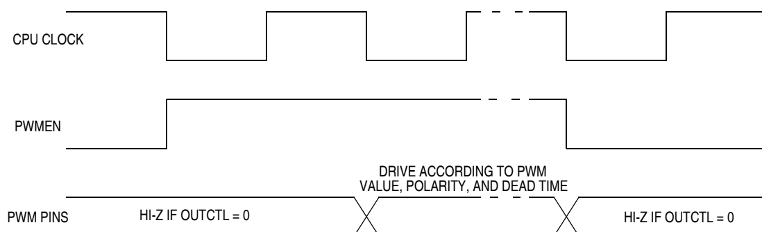
Figure 9-31. PWMEN and PWM Pins
