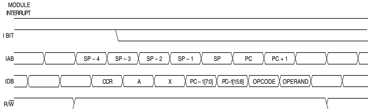
Figure 7-9. Interrupt Recovery
