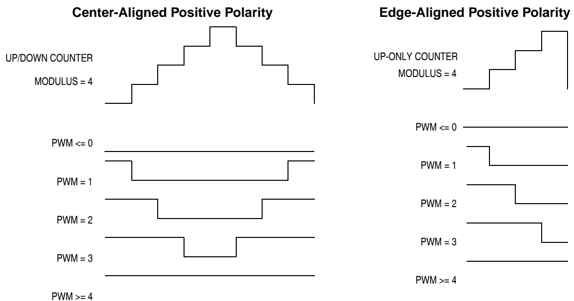
Figure 9-20. PWM Polarity
