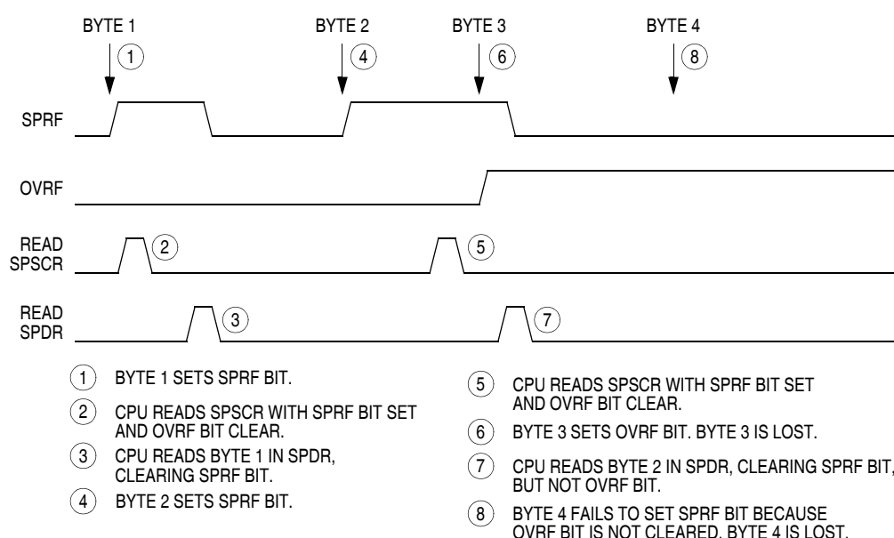
Figure 13-8. Missed Read of Overflow Condition
