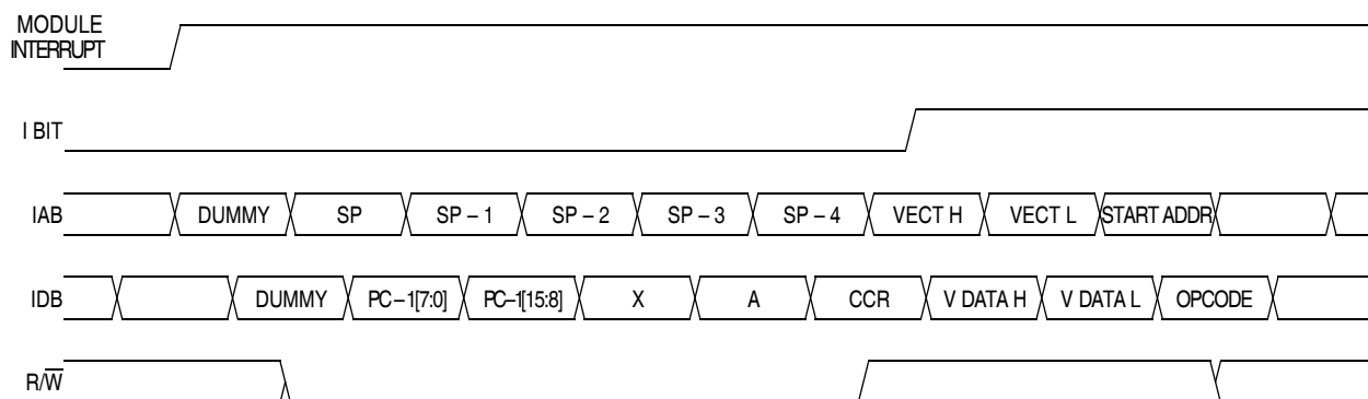
Figure 7-7. Interrupt Entry
