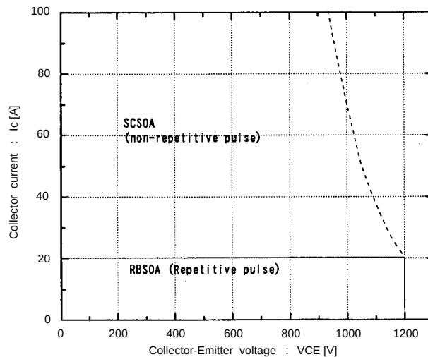
Reversed biased safe operating area +V_{GE}=15V , -V_{GE} \leq 15V , T_J \leq 125^\circ C , R_G \geq 62 \text{ ohm}
