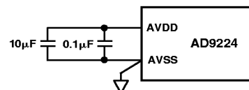
Figure 41. Analog Supply Decoupling
