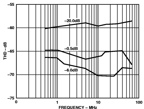
Figure 7. THD vs. Input Frequency (Input Span = 2.0 V p-p, V_{CM} = 2.5 V Differential Input)
