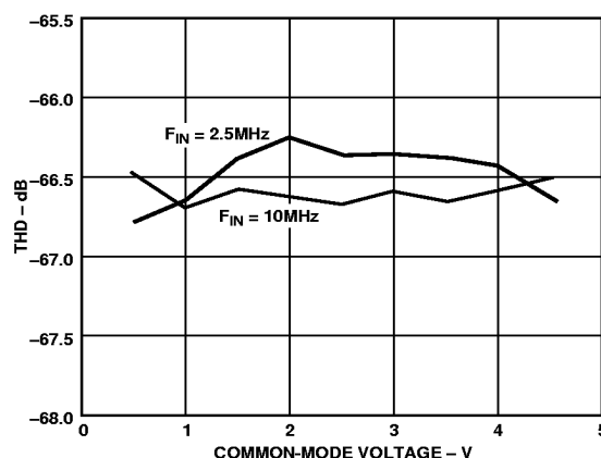
Figure 25a. Common-Mode Voltage vs. THD ( A_{IN} = 2 V Differential)
