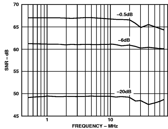
Figure 12. SNR vs. Input Frequency (Input Span = 4.0 V p-p, V_{CM} = 2.5 V Single-Ended Input)
