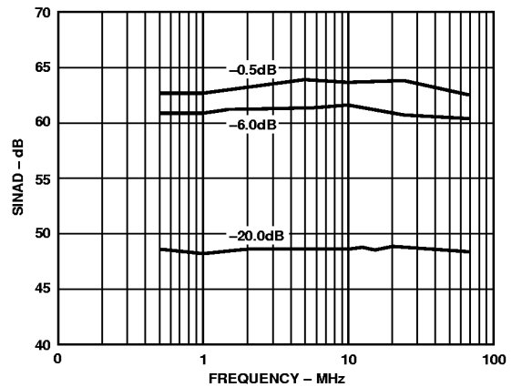
Figure 6. SINAD vs. Input Frequency (Input Span = 2.0 V p-p, V_{CM} = 2.5 V Differential Input)
