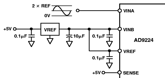
Figure 30. Input Range = 0 V to 2 \times V_{REF}
