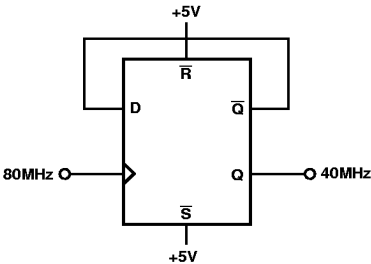
Figure 33. Divide-by-Two Clock Circuit
