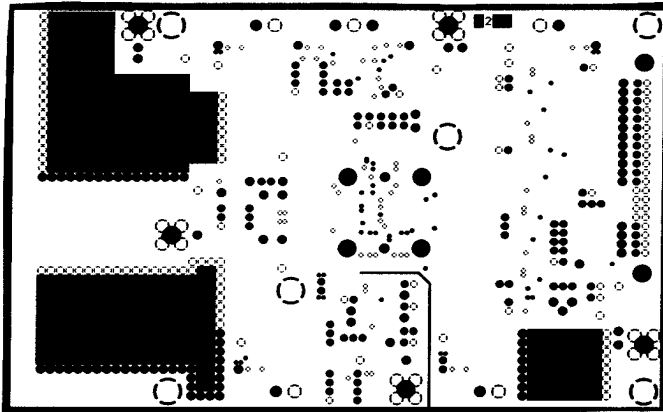
Figure 46. Evaluation Board Ground Plane Layout (Not to Scale)
