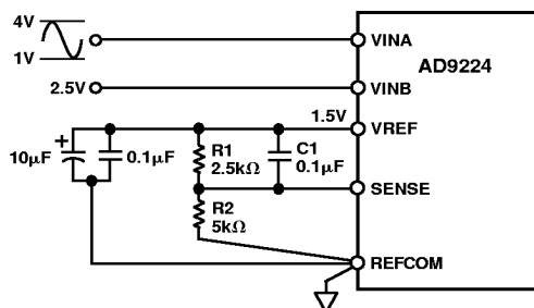
Figure 28. Resistor Programmable Reference—3 V p-p Input Span, V_{CM} = 2.5\text{ V}
