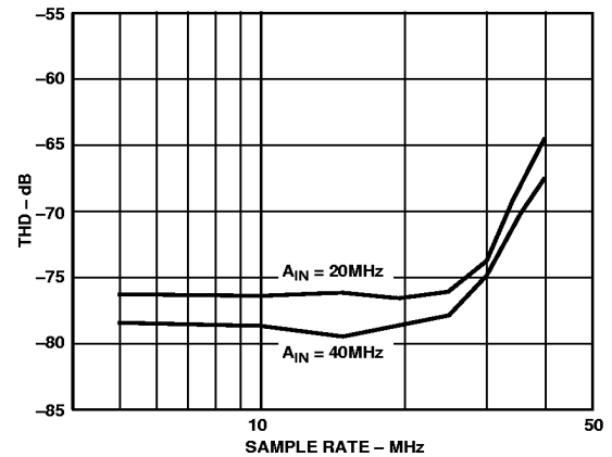
Figure 11. THD vs. Sample Rate ( A_{IN} = -0.5 dB, V_{CM} = 2.5 V (Input Span = 4.0 V p-p, V_{CM} = 2.5 V Differential Input)
