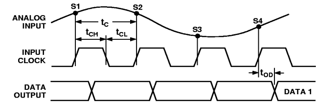
Figure 1. Timing Diagram
