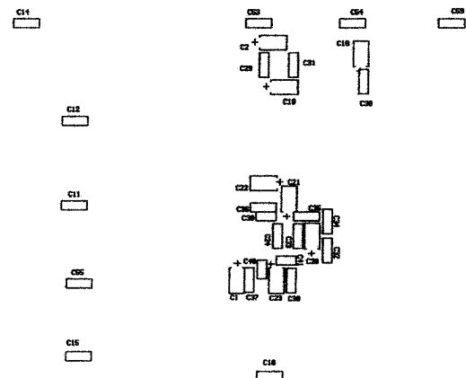
Figure 50. Evaluation Board Solder Side Silkscreen (Not to Scale)
