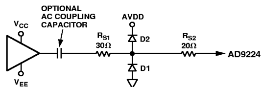
Figure 18. Simple Clamping Circuit
