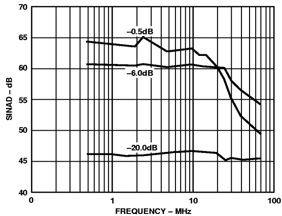
Figure 3. SINAD vs. Input Frequency (Input Span = 4.0 V p-p, V_{CM} = 2.5 V Differential Input)
