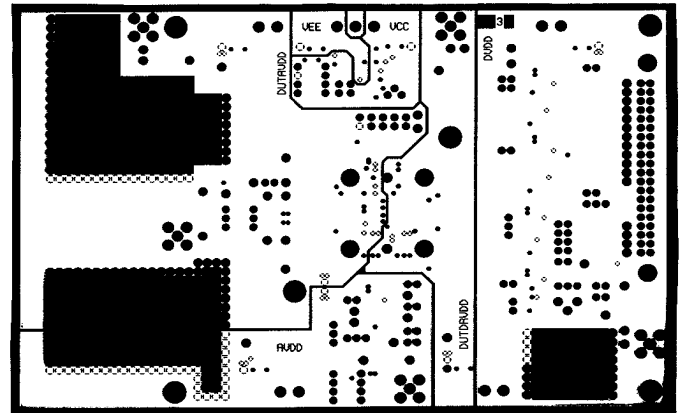
Figure 49. Evaluation Board Power Plane Layout (Not to Scale)
