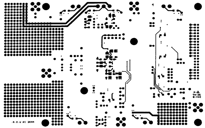
Figure 48. Evaluation Board Solder Side Layout (Not to Scale)
