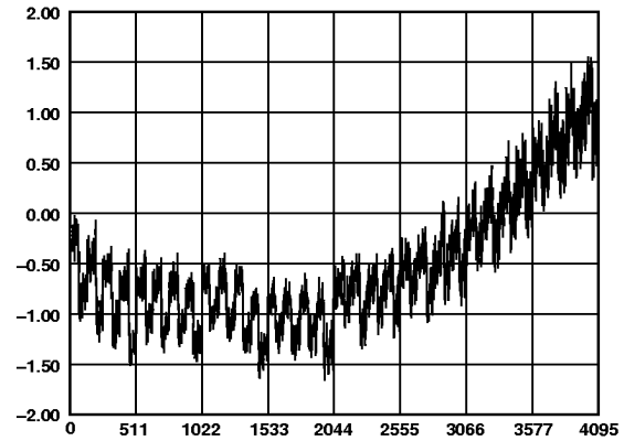
Figure 5. Typical INL
