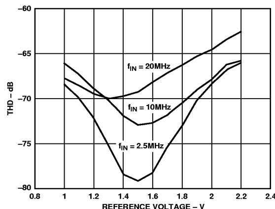
Figure 26b. THD vs. Reference Voltage
