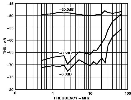
Figure 9. THD vs. Input Frequency (Input Span = 4.0 V p-p, V_{CM} = 2.5 V Single-Ended Input)
