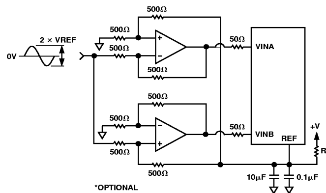
Figure 23. Direct Coupled Drive Circuit with AD8056 Dual Op Amps
