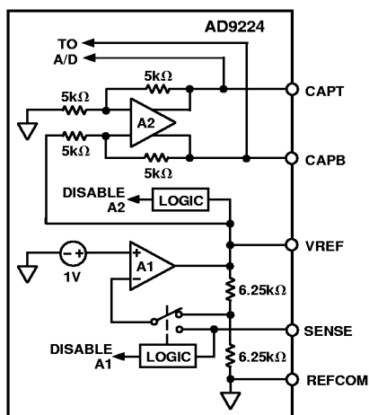
Figure 16. Equivalent Reference Circuit
