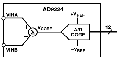
Figure 13. Equivalent Functional Input Circuit
