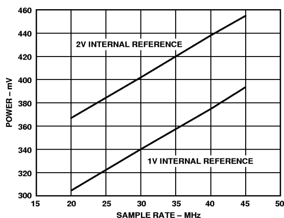
Figure 34. Power Consumption vs. Clock Rate
