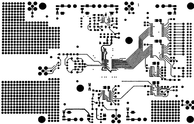
Figure 45. Evaluation Board Component Side Layout (Not to Scale)
