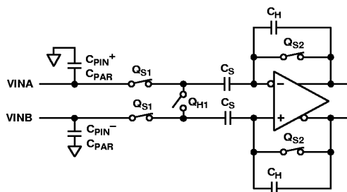
Figure 14. Simplified Input Circuit
