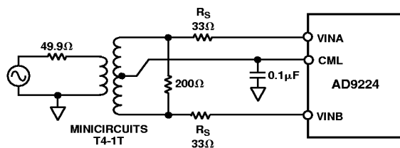
Figure 24. Transformer Coupled Input
