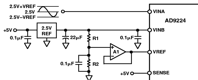
Figure 29. External Reference
