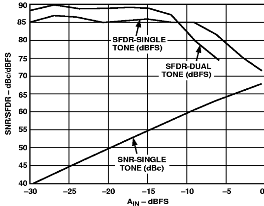
Figure 36. IF Undersampling at 35 MHz ( F_1 = 34.64 MHz, F_2 = 35.43 MHz, f_{\text{CLOCK}} = 28 MSPS)
