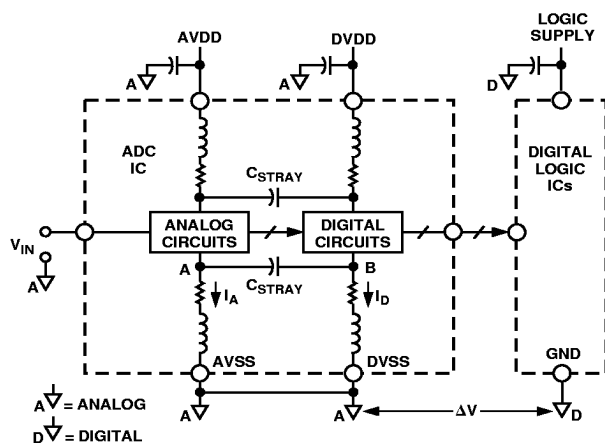
Figure 40. Ground and Power Consideration
