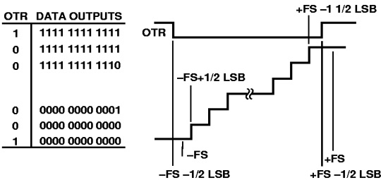
Figure 31. Output Data Format
