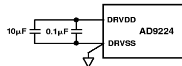
Figure 43. Digital Supply Decoupling
