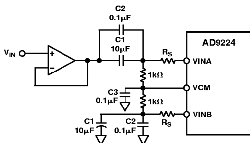
Figure 22. AC-Coupled Input-Flexible Input Span, V_{CM} = 2.5 V
