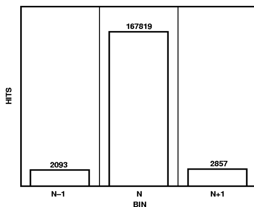
Figure 10. "Grounded-Input" Histogram (Input Span = 2 V p-p)
