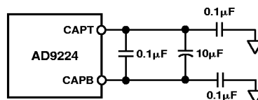
Figure 17. Recommended CAPT/CAPB Decoupling Network
