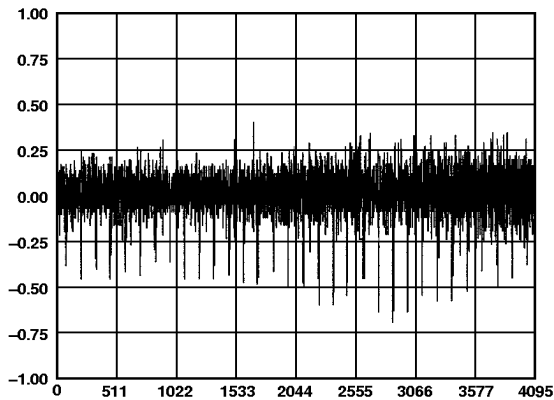
Figure 2. Typical DNL
