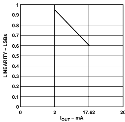
Figure 15. Linearity vs. I_{OUT}
