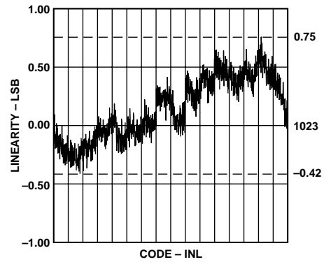
Figure 16. Typical Linearity
