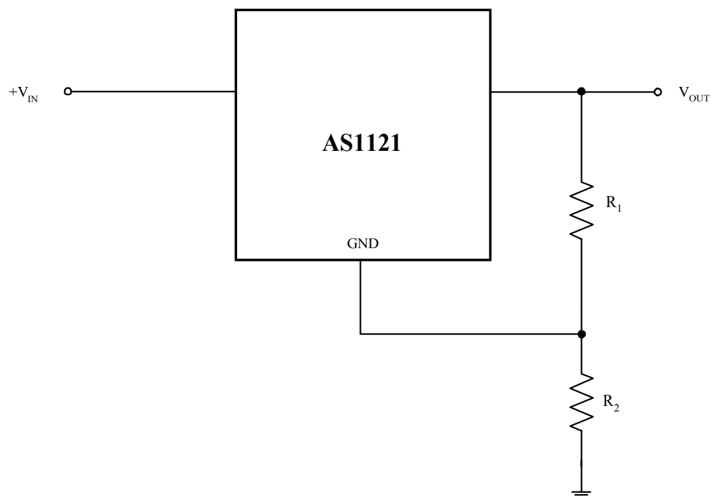
AS1121 ADJUSTABLE REGULATOR
