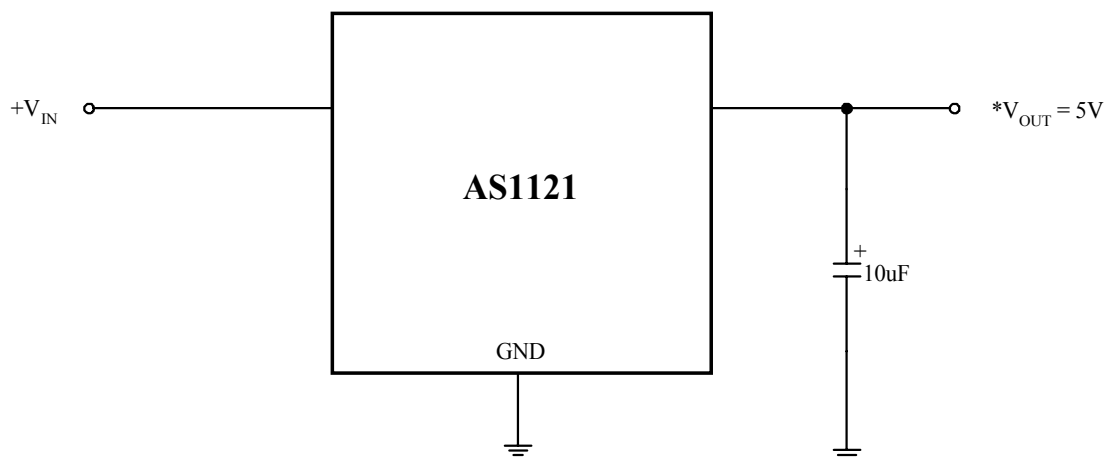
AS1121 FIXED +5V REGULATOR
