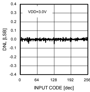
Fig.9 Differential non linearity error
