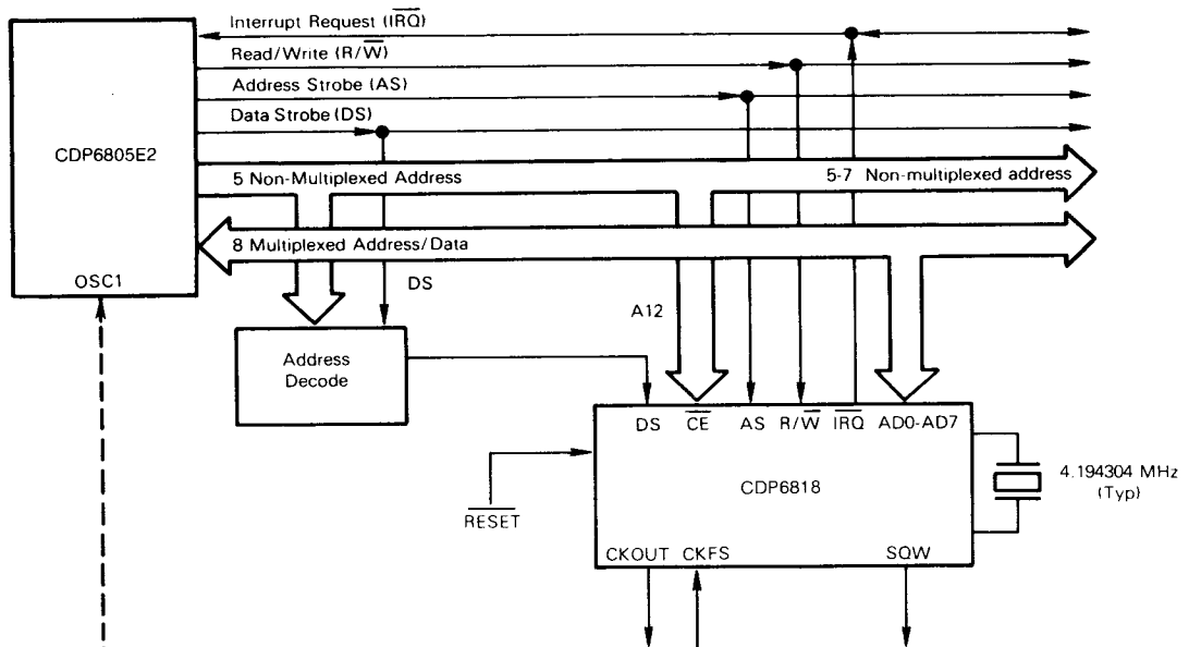
Fig. 19 — CDP6818 interface to CDP6805E2 CMOS multiplexed microprocessor with slow address decoding.
