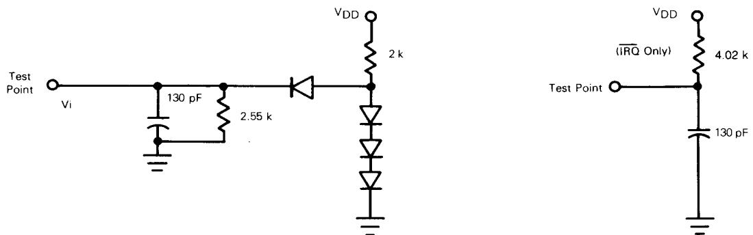
Fig. 6 — TTL equivalent test load.
