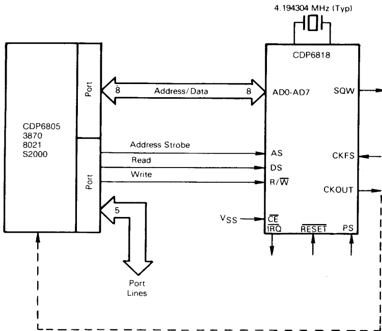
Fig. 20 — CDP6818 interfaced with the ports of a typical single-chip microcomputer.
