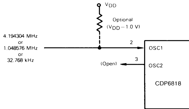
Fig. 10 — External Time-base connection.
