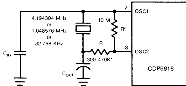
Fig. 10 — External Time-base connection.
