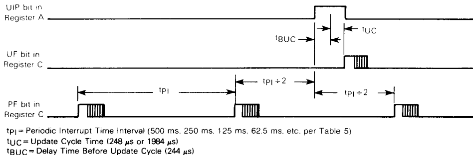
Fig. 16 — Update-ended and periodic interrupt relationships.
