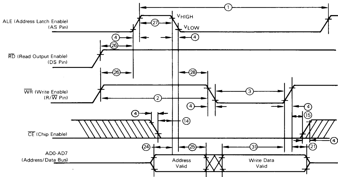
Fig. 4 — Bus-write timing competitor multiplexed bus.
