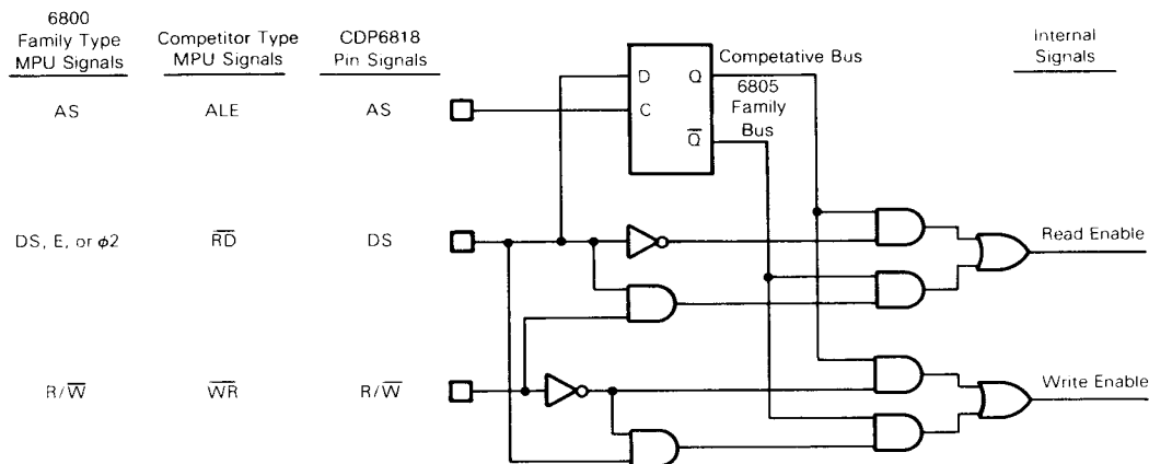
Fig. 9 — Functional diagram of MOTEL circuit.
