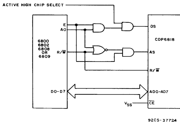
Fig. 21 — CDP6818 interfaced with Motorola type processors
