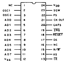
PACKAGE TYPES D AND E TOP VIEW
