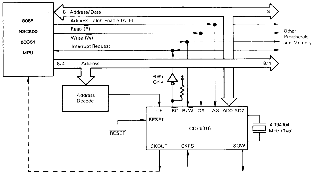
Fig. 18 — CDP6818 interfaced to competitor compatible multiplexed bus microprocessors.
