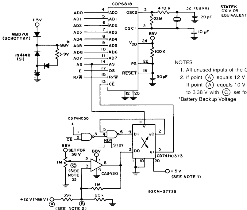
Fig. 23 — Typical Application Circuit
