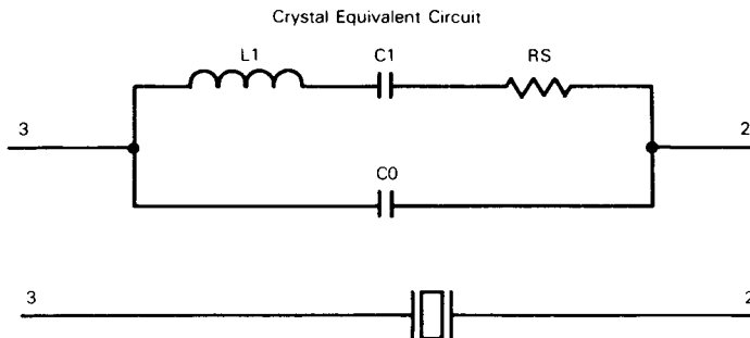
Fig. 11 — Crystal oscillator connection.
