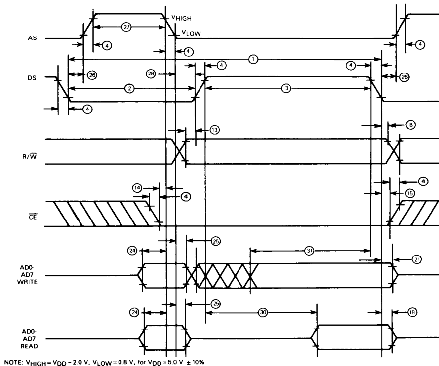
Fig. 2 — CDP6818 bus timing waveforms.
