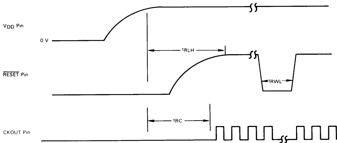
Fig. 7 — Power-up timing waveforms.
