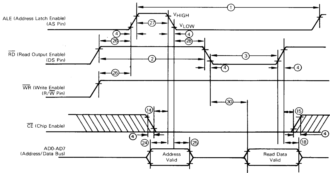
Fig. 3 — Bus-read timing competitor multiplexed bus.
