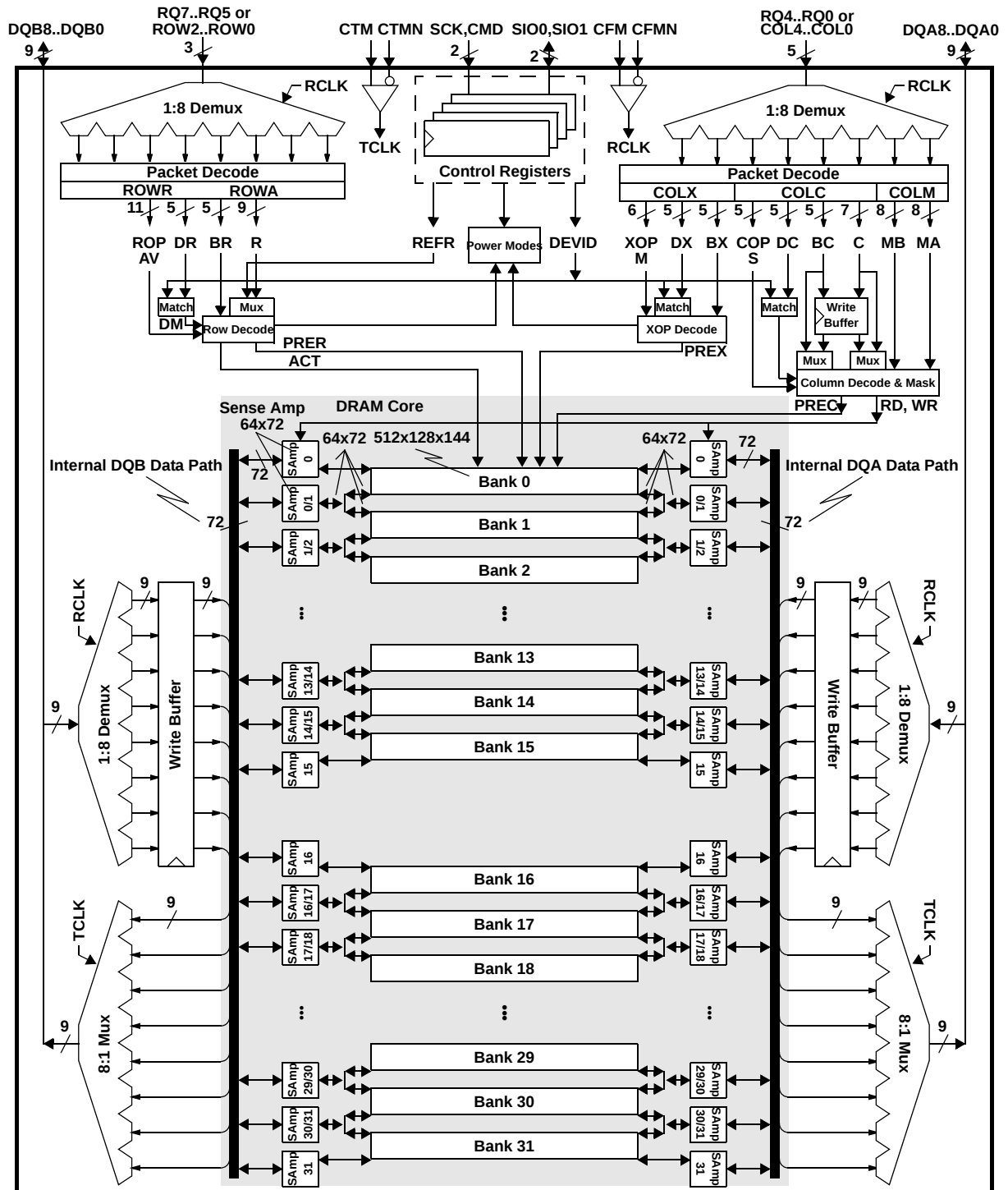
Figure 2: 256/288-Mbit (512Kx16/18x32s) RDRAM Device Block Diagram
