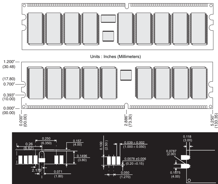
Figure 1: KVR266X72RC25L/2G 184-Pin DDR SDRAM Module
