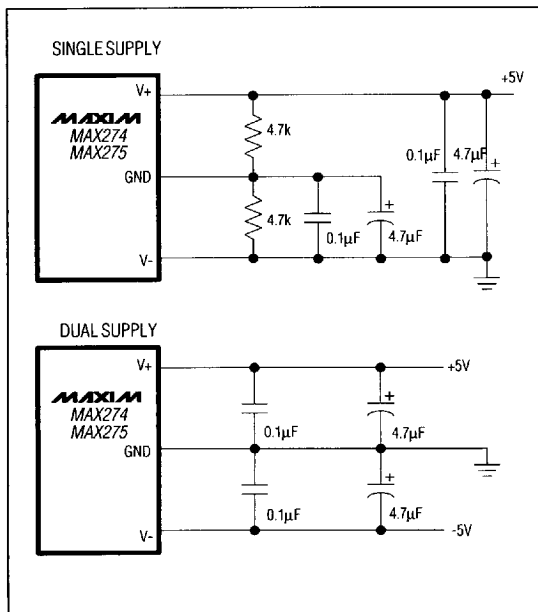
Figure 9. Power-Supply Configurations
