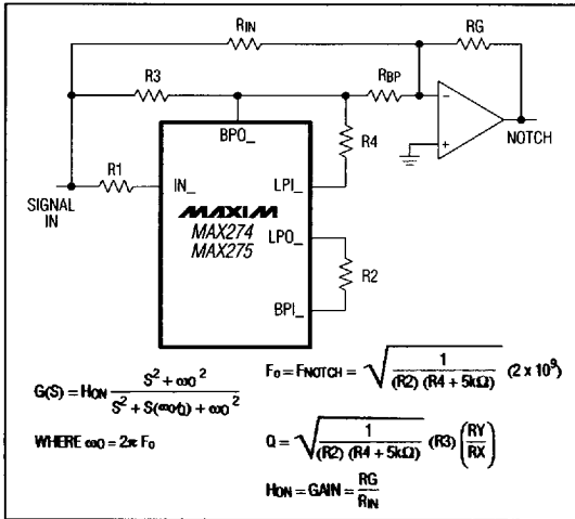
Figure 6a. Creating a Notch Output
