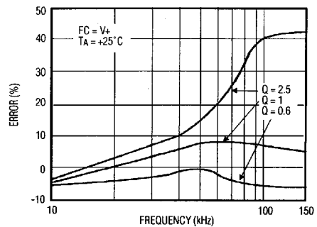
Q ERROR vs. FREQUENCY
