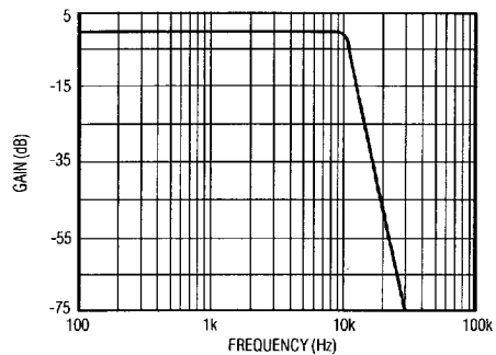
FILTER RESPONSE USING TYPICAL OPERATING CIRCUIT
