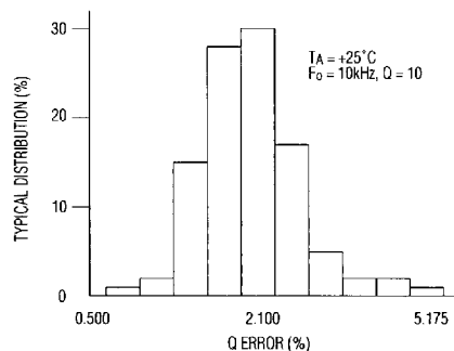
TYPICAL DISTRIBUTION OF Q ERRORS
