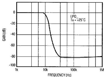
FILTER WIDEBAND RESPONSE USING TYPICAL OPERATING CIRCUIT
