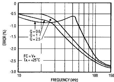
F0 ERROR vs. FREQUENCY
