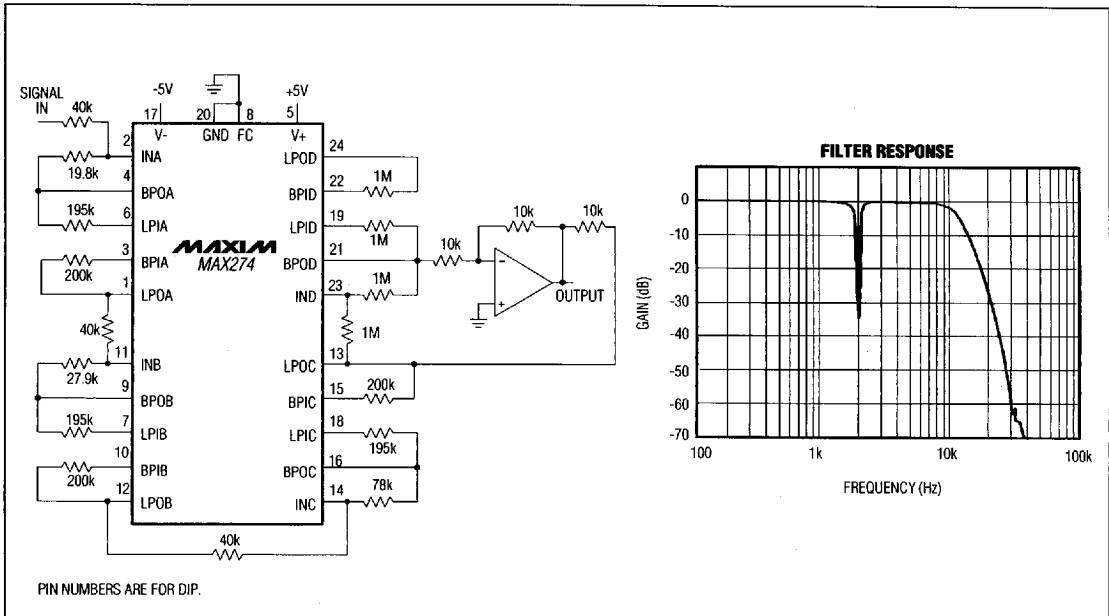
Figure 11. 10kHz 6th-Order Butterworth Lowpass Filter with 2kHz Notch (MAX274)
