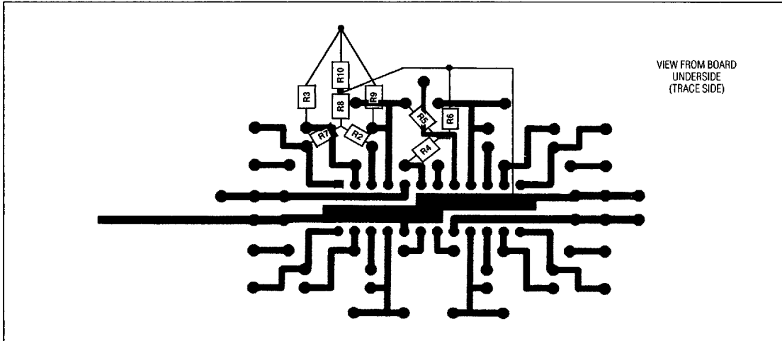
Figure 3. T-Network PC Board Connections
