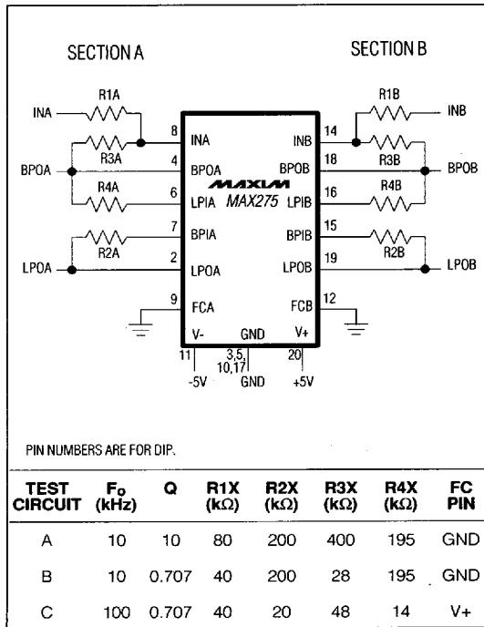
Figure 1b. MAX275 Connection Diagram and Test Circuit
