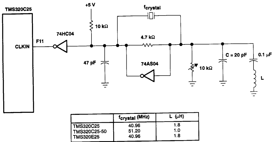
Figure 7. External Clock Option
