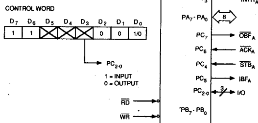
MODE 2 AND MODE 1 (INPUT)
