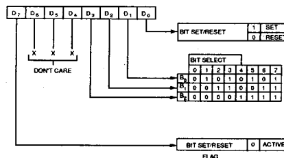
Figure 9 : BIT SET/RESET FORMAT
