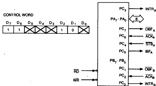
MODE 2 AND MODE 1 (OUTPUT)
