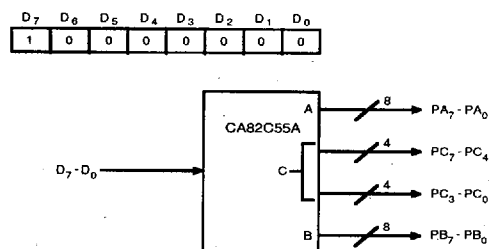
Figure 10 : MODE 0 CONFIGURATION
