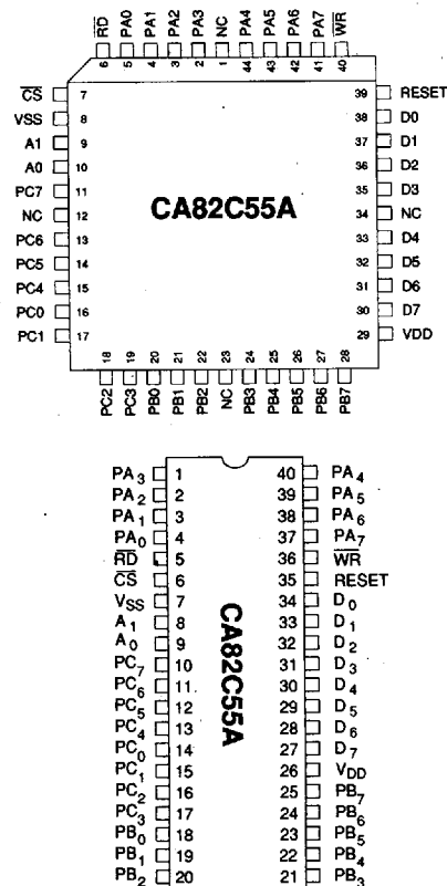
Figure 2 : PLCC and DIP PIN CONFIGURATIONS
