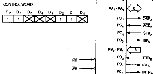
Figure 16 : MODE 1/4 COMBINATIONS
