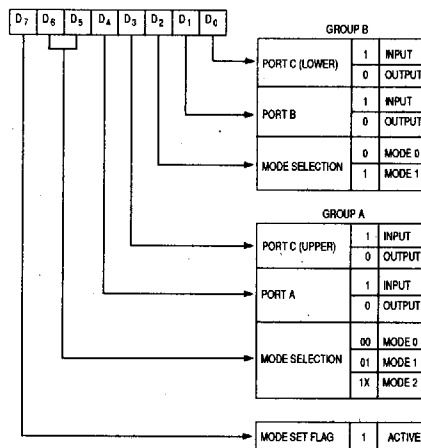
Figure 8 : MODE DEFINITION FORMAT
