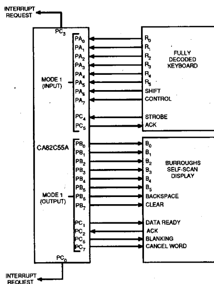
Figure 20 : KEYBOARD and DISPLAY INTERFACE
