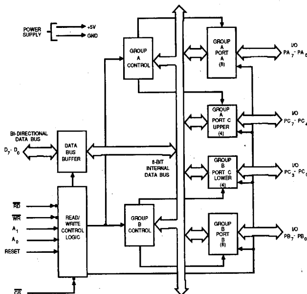
Figure 1 : CA82C55A BLOCK DIAGRAM
