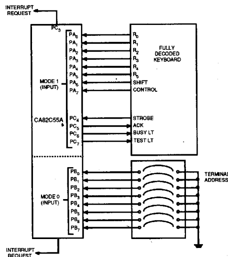
Figure 21 : KEYBOARD and TERMINAL ADDRESS INTERFACE
