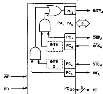
Figure 15 : MODE 2
