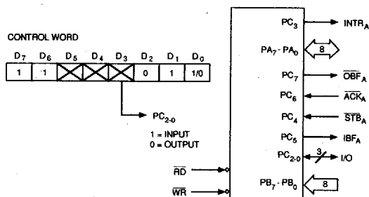
MODE 2 AND MODE 0 (INPUT)
