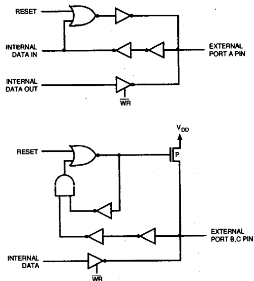
Figure 3 : PORTs A, B & C BUS-HOLD CONFIGURATION
