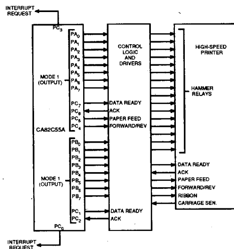
Figure 19 : PRINTER INTERFACE
