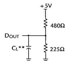
Figure 1. Output Load
