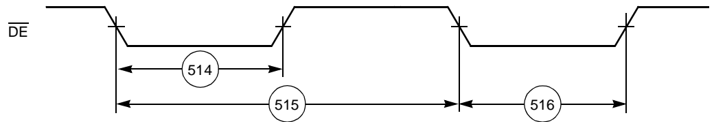
Figure 2-48. OnCE—Debug Request
