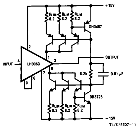
FIGURE 6. LH0063 Current Limiting Using Current Sources
