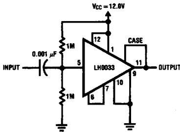
Single Supply AC Amplifier
