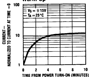
LH0033 Normalized Input Bias Current During Warm-Up
