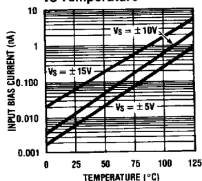
LH0033 Input Bias Current vs Temperature
