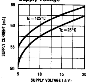
LH0063 Supply Current vs Supply Voltage
