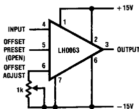
FIGURE 2. Offset Zero Adjust for LH0063
