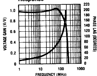
LH0063 Frequency Response
