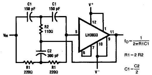
4.5 MHz Notch Filter
