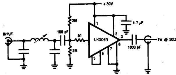
1W CW Final Amplifier
