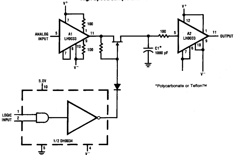
High Speed Sample and Hold
