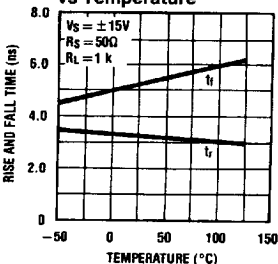
LH0033 Rise and Fall Time vs Temperature
