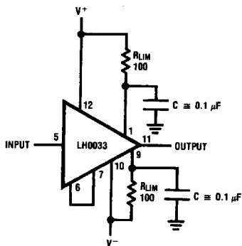
FIGURE 3. LH0033 Using Resistor Current Limiting
