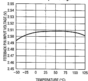
Feedback Pin Input Voltage
