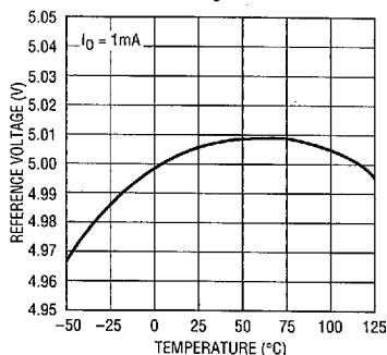
Reference Voltage
