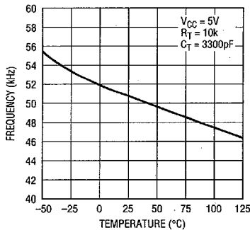
Oscillator Frequency
