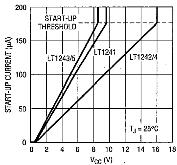
Start-Up Current
