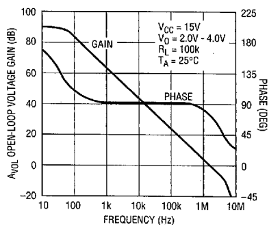
Error Amplifier Open-Loop Gain and Phase
