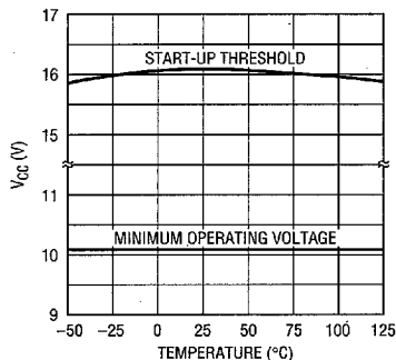
Undervoltage Lockout – LT1242, LT1244
