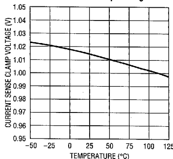
Current Sense Clamp Voltage
