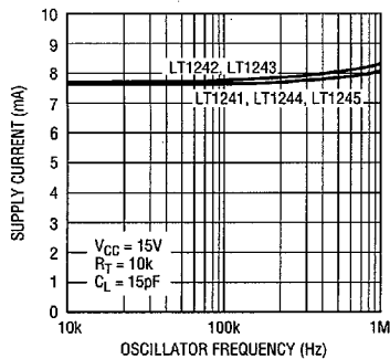
Supply Current vs Oscillator Frequency
