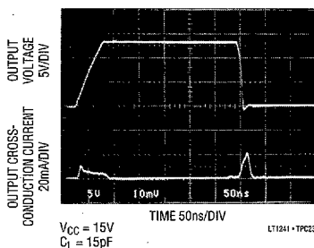
Output Cross-Conduction Current
