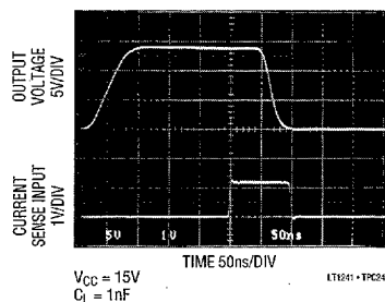
Current Sense Delay
