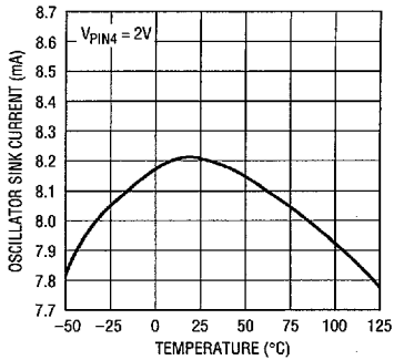
Oscillator Sink Current
