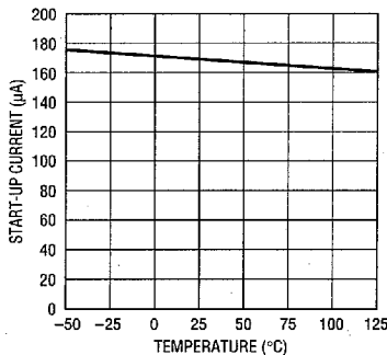
Start-Up Current
