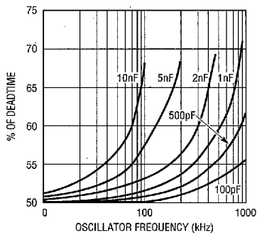
Output Deadtime vs Oscillator Frequency – LT1241, LT1243, LT1245
