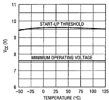
Undervoltage Lockout – LT1241
