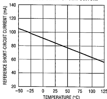
Reference Short-Circuit Current
