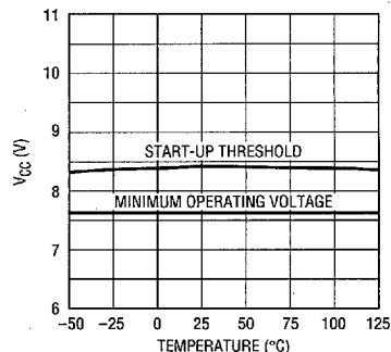
Undervoltage Lockout – LT1243, LT1245
