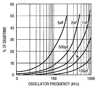
Output Deadtime vs Oscillator Frequency – LT1242, LT1244
