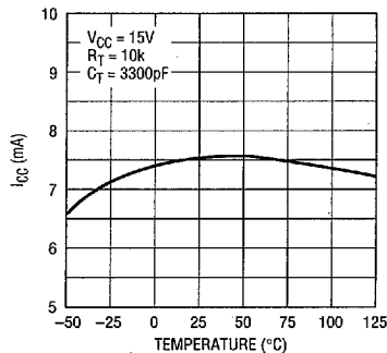
Supply Current
