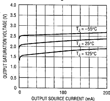
High Level Output Saturation Voltage
