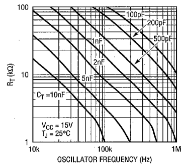
Timing Resistor vs Oscillator Frequency
