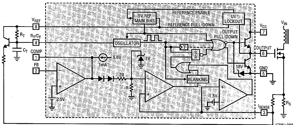
Slope Compensation at I_{SENSE} Pin
