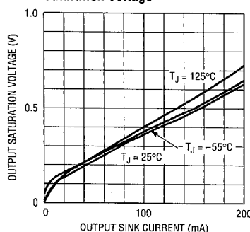
Low Level Output Saturation Voltage
