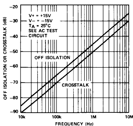
CROSSTALK AND "OFF" ISOLATION vs FREQUENCY
