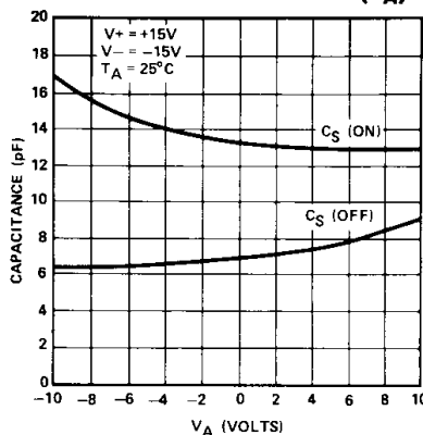
SWITCH CAPACITANCES vs ANALOG VOLTAGE ( V_A )
