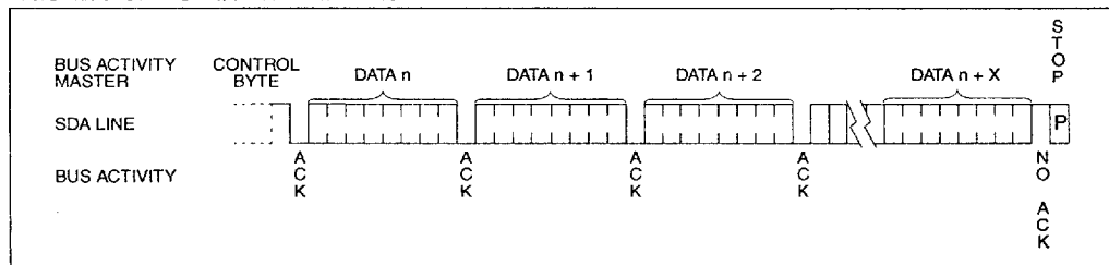
FIGURE 7-3: SEQUENTIAL READ
