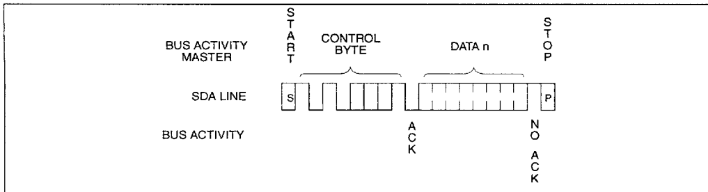
FIGURE 7-2: RANDOM READ
