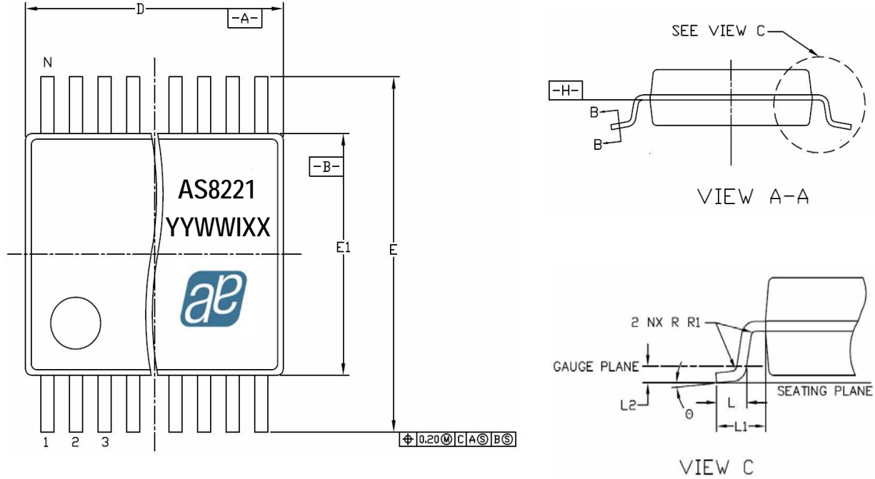
Figure 20. Package Drawings and Dimensions
