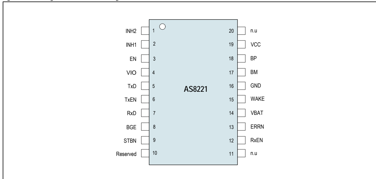
Figure 2. Pin Assignments SSOP20 Package
