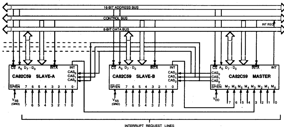
Figure 25 : MULTIPLE CA82C59As IN A CASCADED SYSTEM
