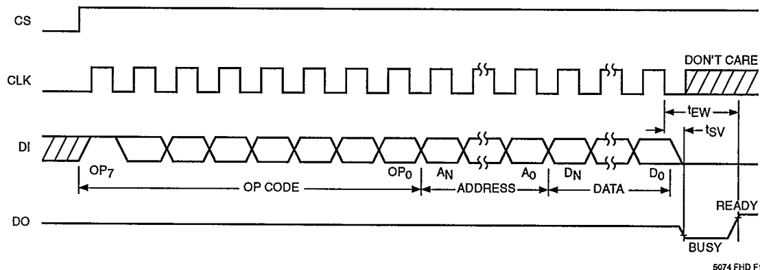
Figure 8. Write Timing
