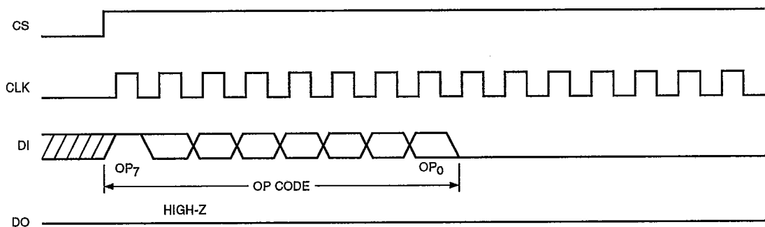
Figure 9. EWEN/EWDS Timing
