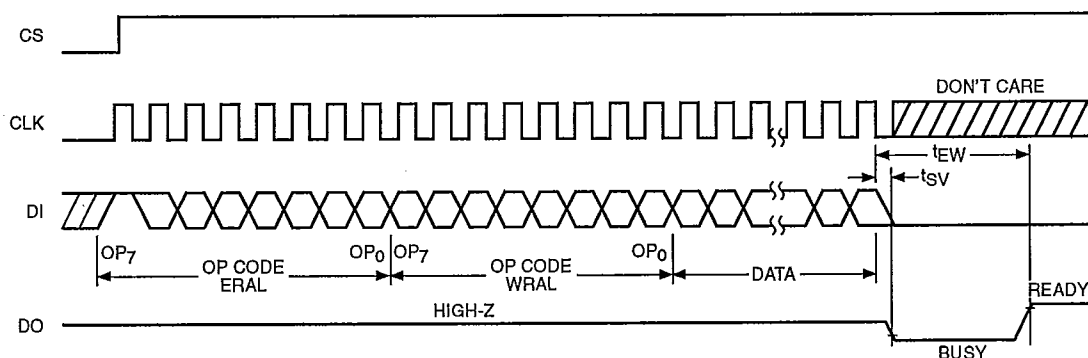
Figure 12. WRAL Timing
