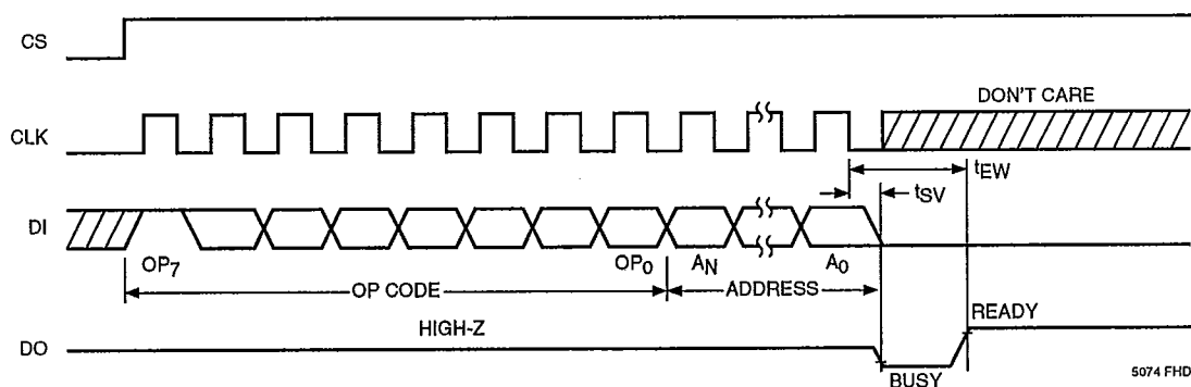
Figure 10. Erase Timing
