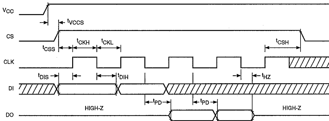
Figure 1. A.C. Timing
