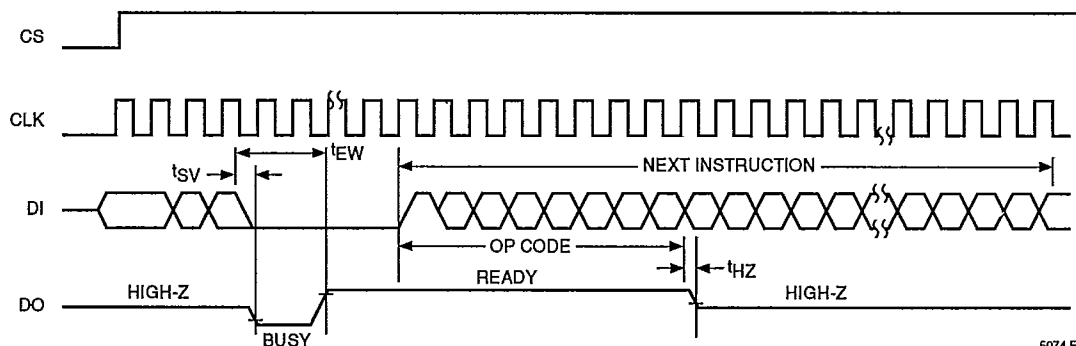
Figure 13. Next Instruction Timing (9)
