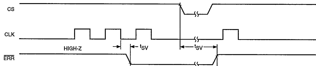
Figure 4. ERR Pin Timing
