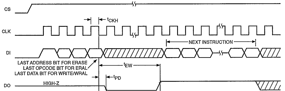
Figure 5. Program/Erase Timing
