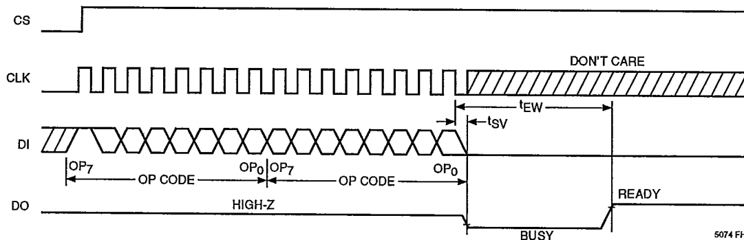
Figure 11. ERAL Timing
