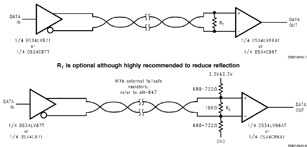
FIGURE 6. Typical Driver Connection
