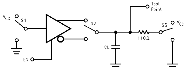
FIGURE 4. Driver Single-Ended TRI-STATE Test Circuit
