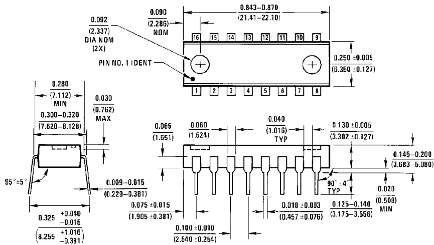
16-Lead Molded Dual-In-Line Package (N) Order Number DS34LV87TN NS Package Number N16A
