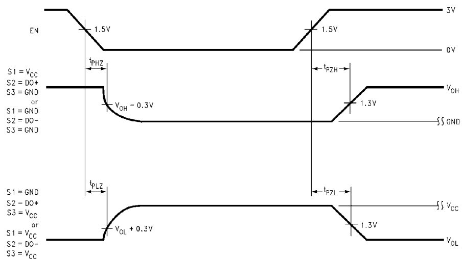
FIGURE 5. Driver Single-Ended TRI-STATE Waveforms
